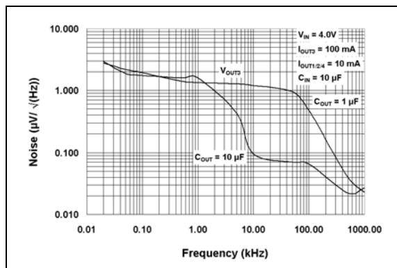
FIGURE 2-24: Output Noise.
