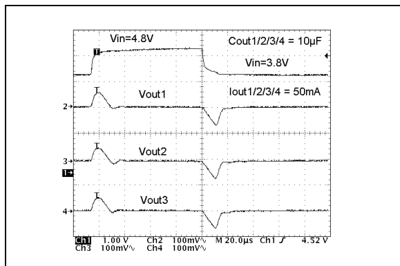
FIGURE 2-20: Line Step Response.
