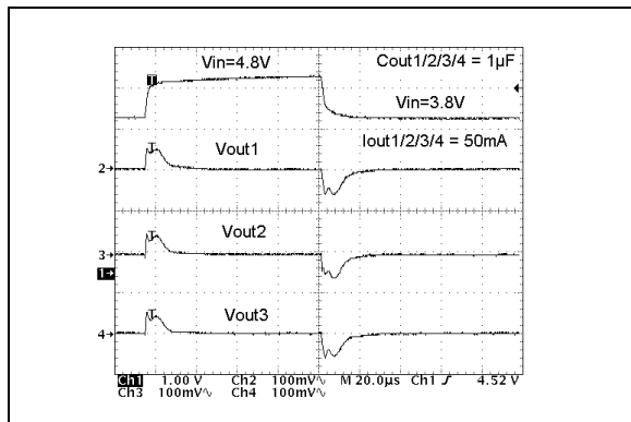
FIGURE 2-19: Line Step Response.
