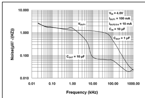
FIGURE 2-23: Output Noise.
