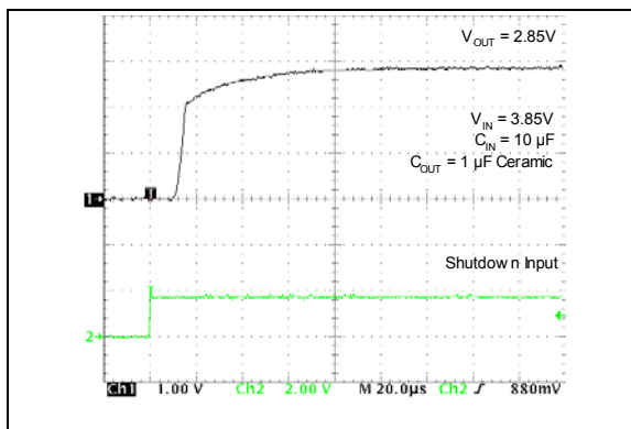
FIGURE 2-20: Wake-Up Response.
