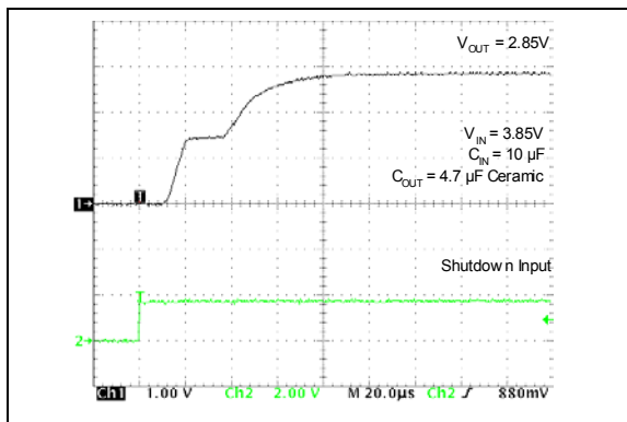
FIGURE 2-21: Wake-Up Response.
