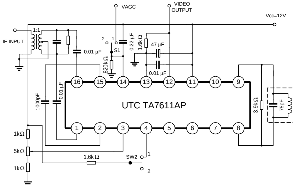
TEST CIRCUIT 2
