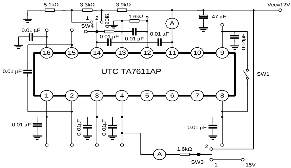
TEST CIRCUIT 2
