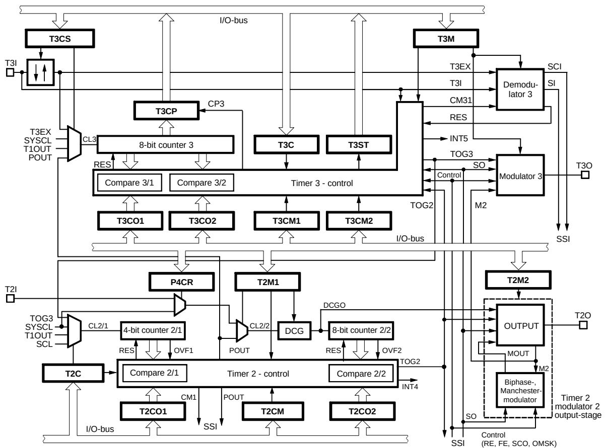
Figure 83. Combination Timer 3 and Timer 2
