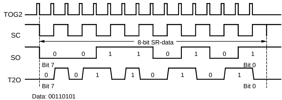
Figure 75. Manchester Modulation 1
