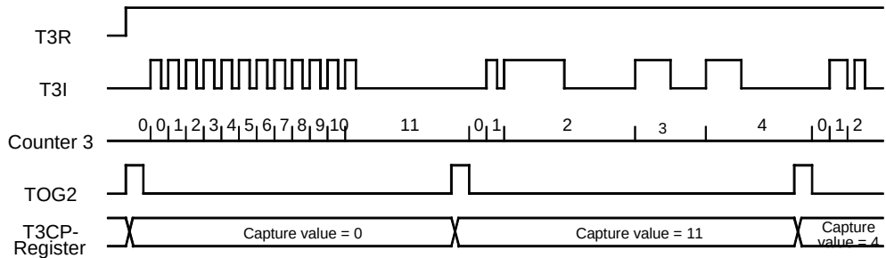
Figure 55. Event Counter with Time Gate
