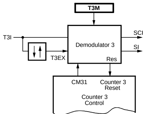
Figure 62. Timer 3 Demodulator 3
