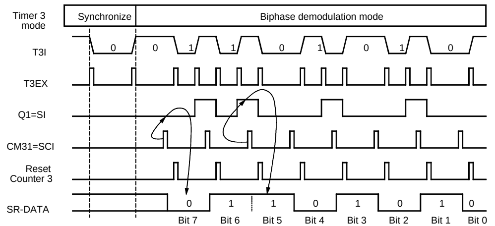
Figure 82. Biphase Demodulation
