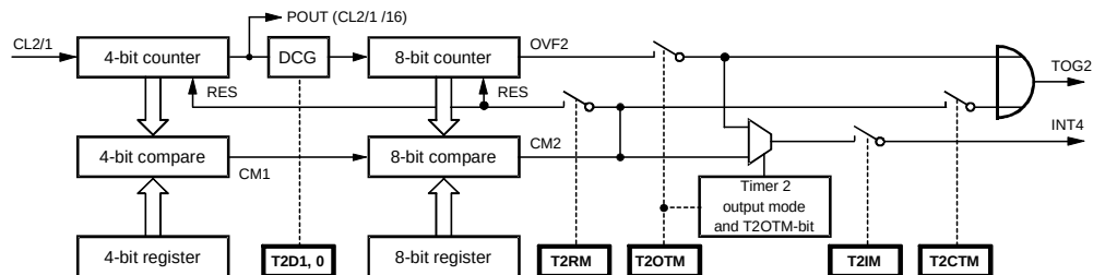
Figure 36. 12-bit Compare Counter
