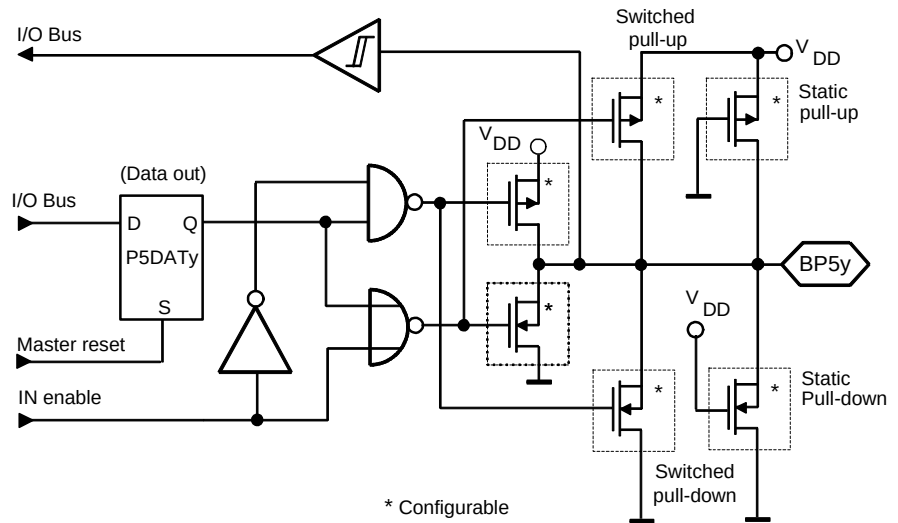
Figure 29. Bi-directional Port 5
