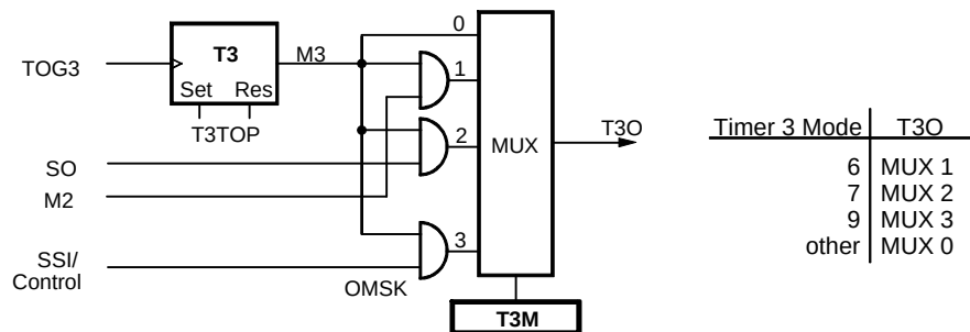
Figure 61. Modulator 3
