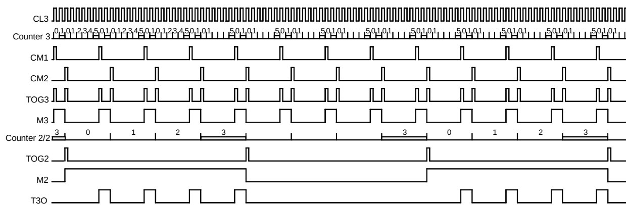
Figure 86. Burst Modulation 1
