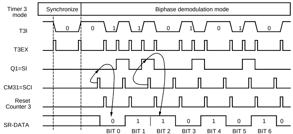
Figure 59. Biphase Demodulation
