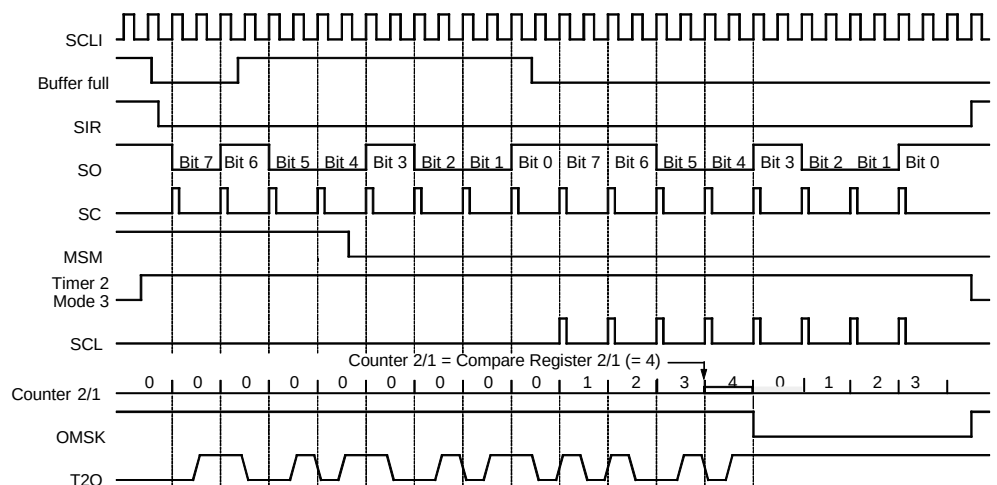
Figure 76. Manchester Modulation 2
