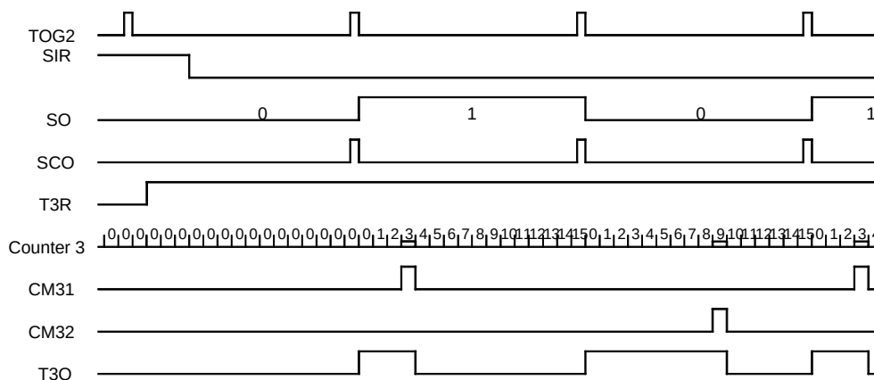
Figure 57. Pulse-width Modulation
