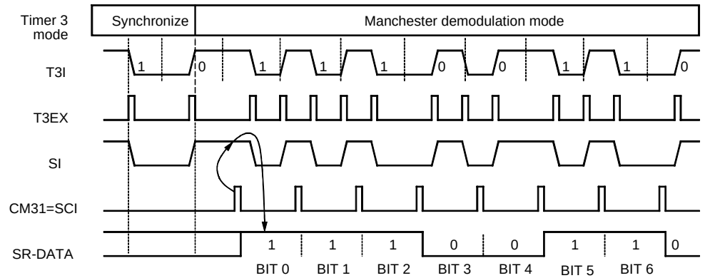
Figure 58. Manchester Demodulation
