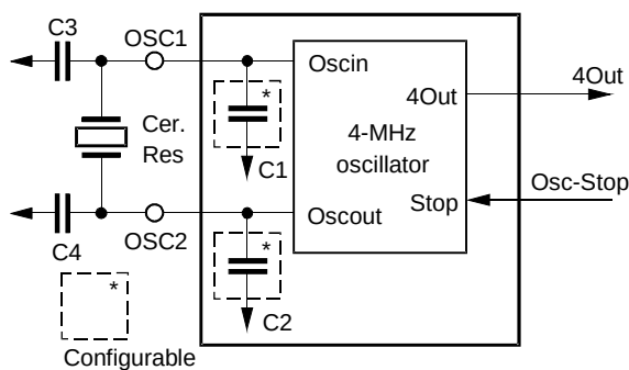
Figure 24. Ceramic Resonator
