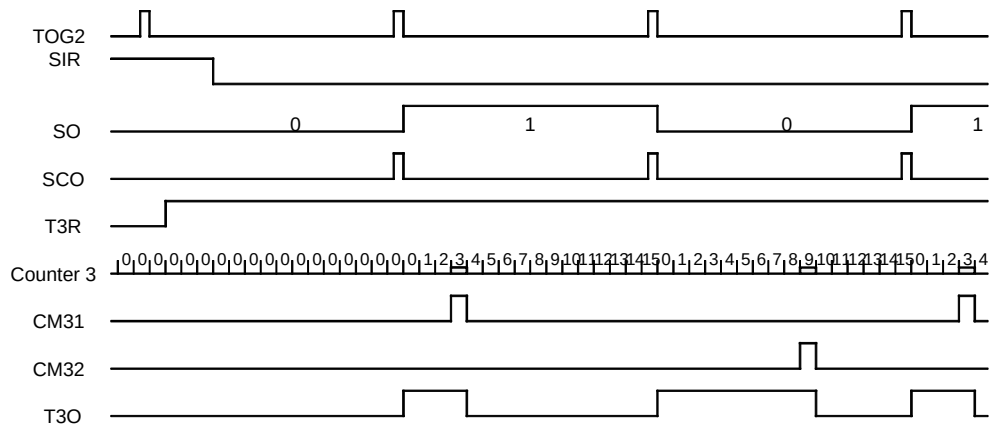
Figure 80. Pulse-width Modulation
