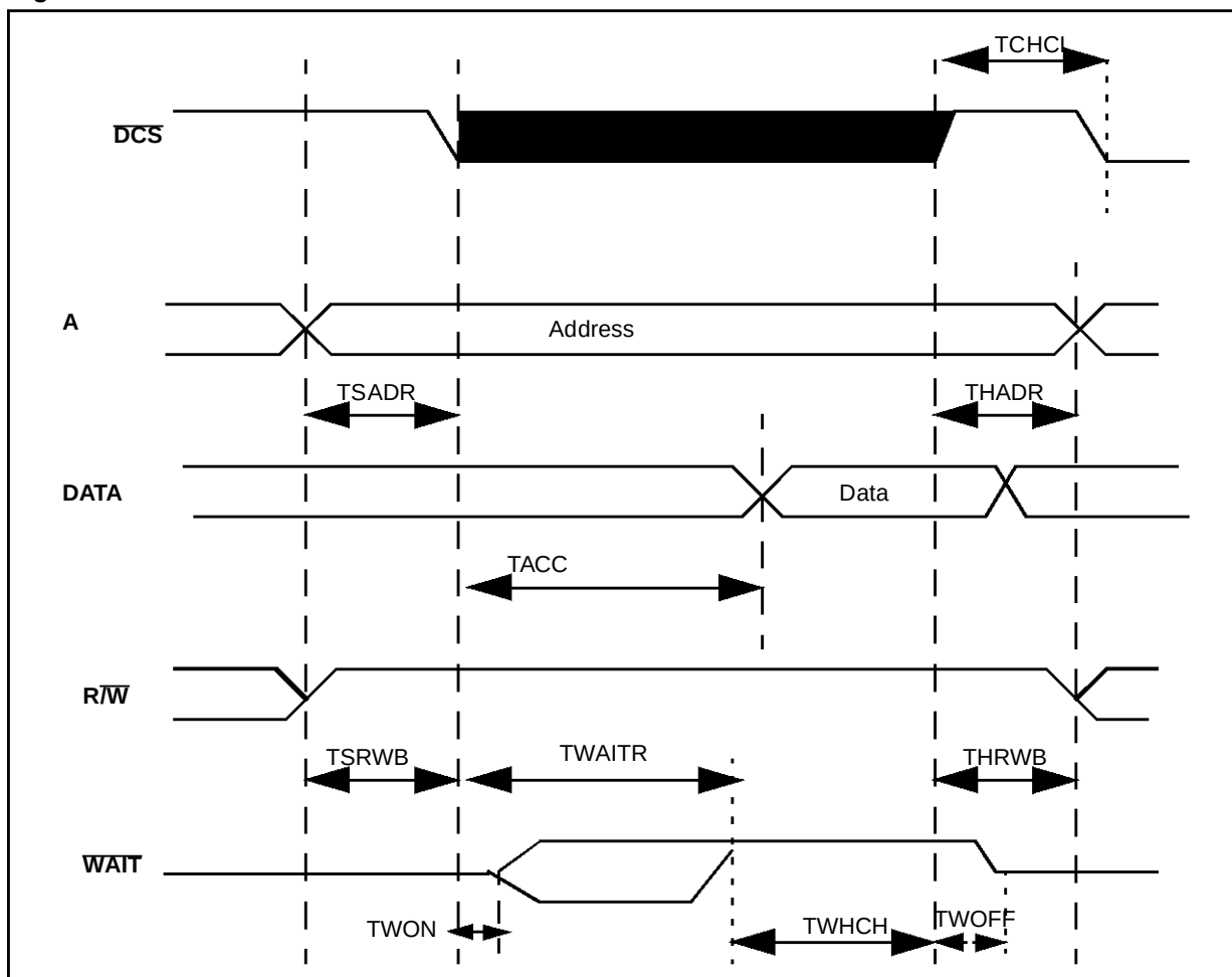
Figure 13. Read Access
