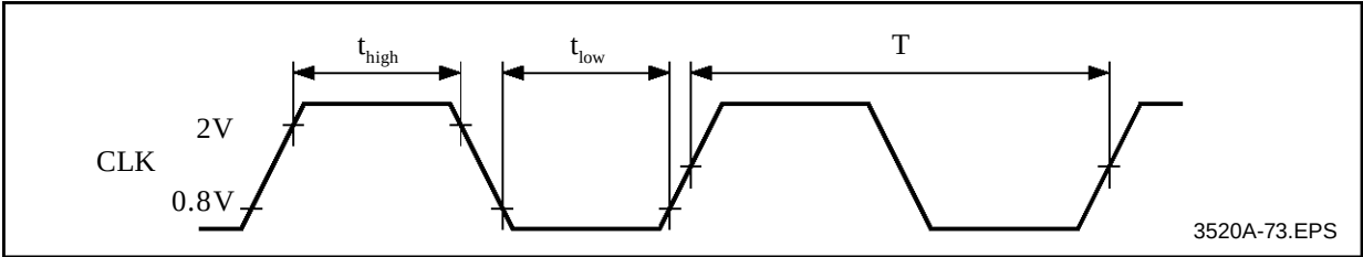
Figure 11. Clock Signals
