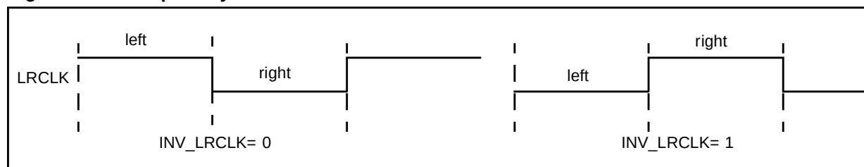
Figure 9. LRCLK polarity
