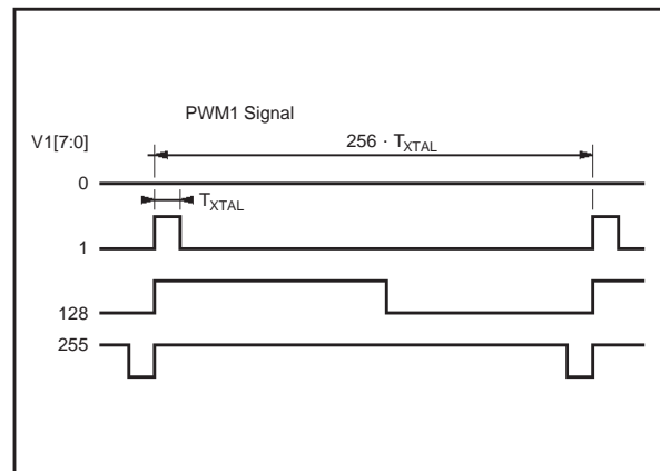
Figure 6 : PWM Timing
