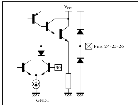
Figure 22 : Pin 30 - ICAT
