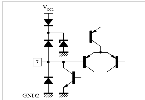
Figure 11 : Pin 7 - SCL
