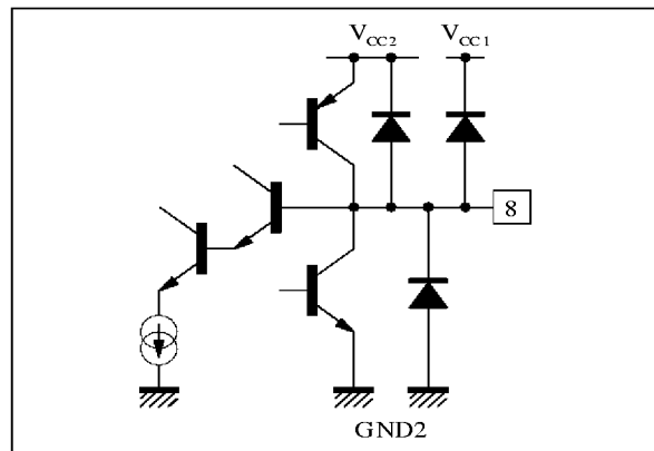
Figure 12 : Pin 8 - FTUN1
