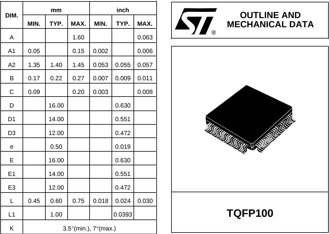
Figure 15: 100TQFP package outline and mechanical data
