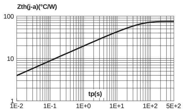
Fig. 14: Variation of thermal impedance junction to ambient versus pulse duration (epoxy printed circuit board FR4, e(\text{Cu})=35\mu\text{m} , S(\text{Cu})=1\text{cm}^2 ).
