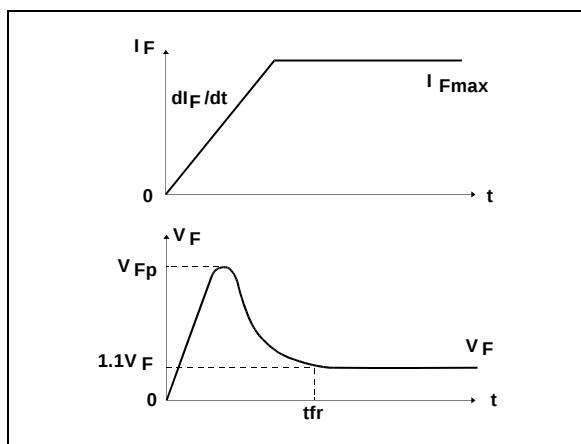
Fig. 8 : TURN-ON CHARACTERISTICS
