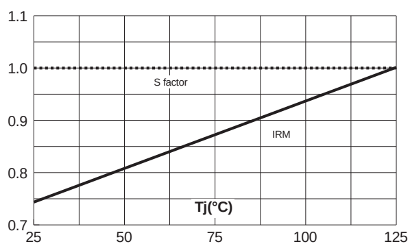
Fig. 6: Relative variation of dynamic parameters versus junction temperature (reference T_J = 125^\circ\text{C} ).
