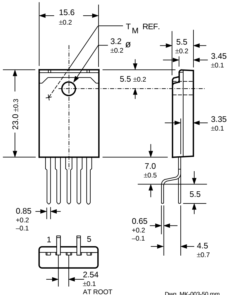
(controlling dimensions)
