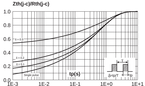
Fig. 6-2: Relative variation of thermal transient impedance junction to case versus pulse duration (ISOWATT220AB / TO-220FPAB).
