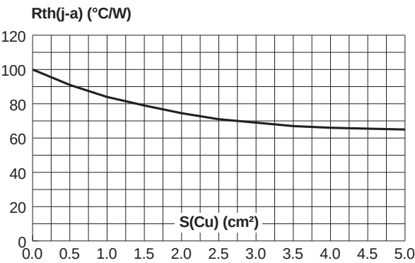
Fig. 10: Thermal resistance junction to ambient versus copper surface under each lead (Epoxy printed circuit board FR4, copper thickness s(Cu) = 35μm)
