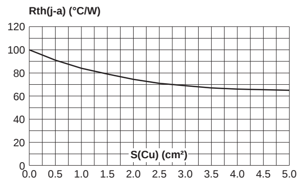
Fig. 8: Thermal resistance junction to ambient versus copper surface under tab (Epoxy printed circuit board FR4, copper thickness: 35μm).
