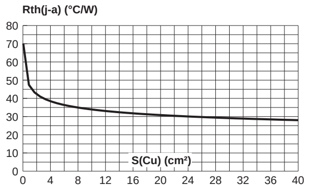
Fig.8 : Thermal resistance junction to ambient versus copper surface under tab (Epoxy printed circuit board FR4, copper thickness : 35 \mu\text{m} ). (STPS20L25G only)
