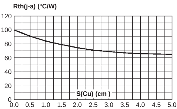
Fig. 8-1: Thermal resistance junction to ambient versus copper surface under tab (Epoxy printed circuit board FR4, copper thickness: 35μm) (SMB).
