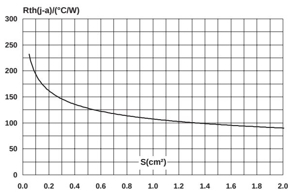
Fig. 10: Thermal resistance junction to ambient versus copper surface under tab (epoxy printed board FR4, \text{Cu} = 35\mu\text{m} ).
