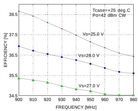
Efficiency vs Frequency
