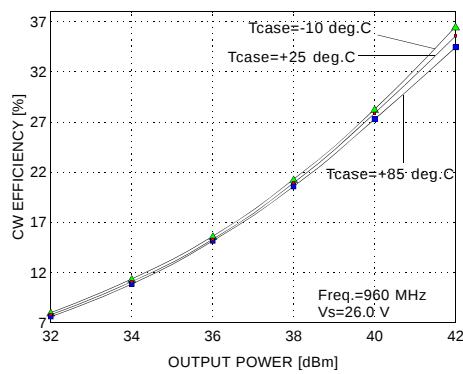
CW Efficiency vs Output Power & Temperature
