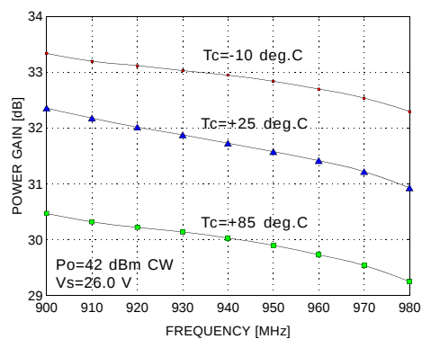
Power Gain vs Frequency &amp; Temperature
