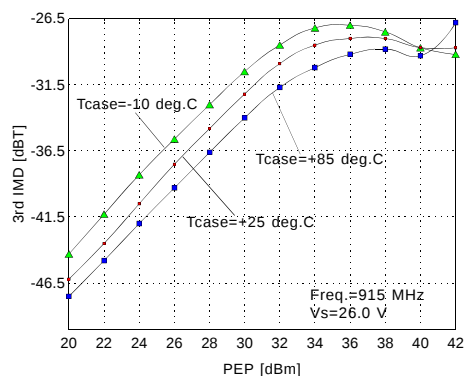
3rd Order IMD vs Output Power &amp; Temperature
