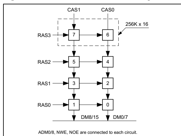
Figure 27 : 256K x 16 DRAM Circuit Organization
