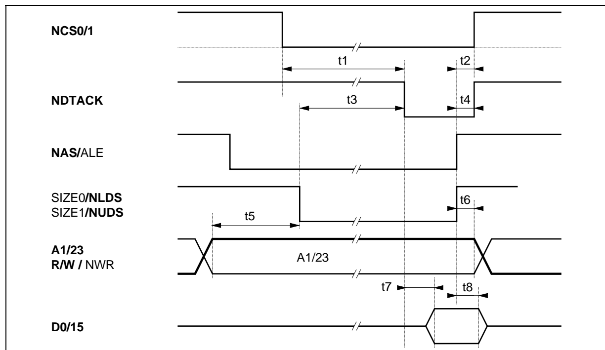
Figure 52 : 68000 Read Cycle
