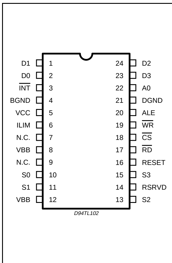
DIP24 PIN CONNECTION (Top view)
