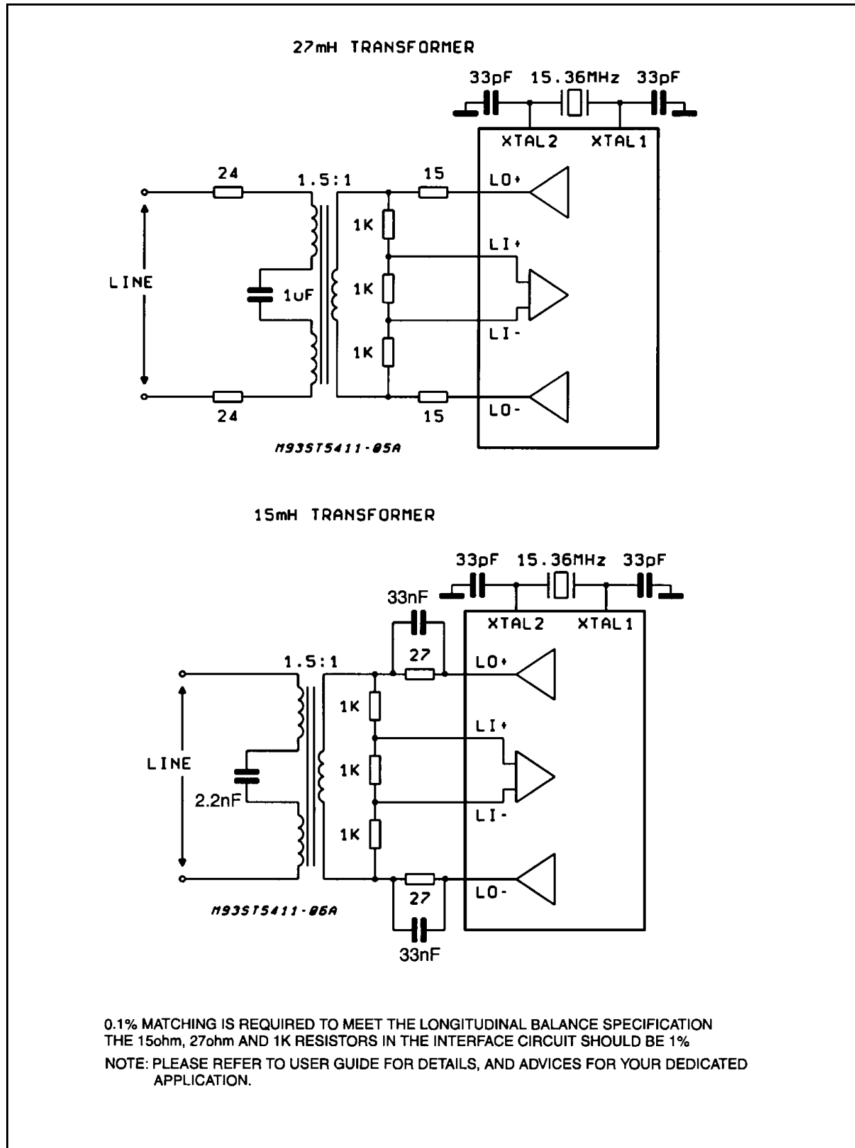
Figure 12: Recommended connections.
