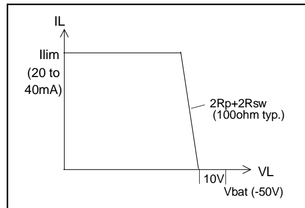
Figure 3. DC characteristic in ACTIVE mode
