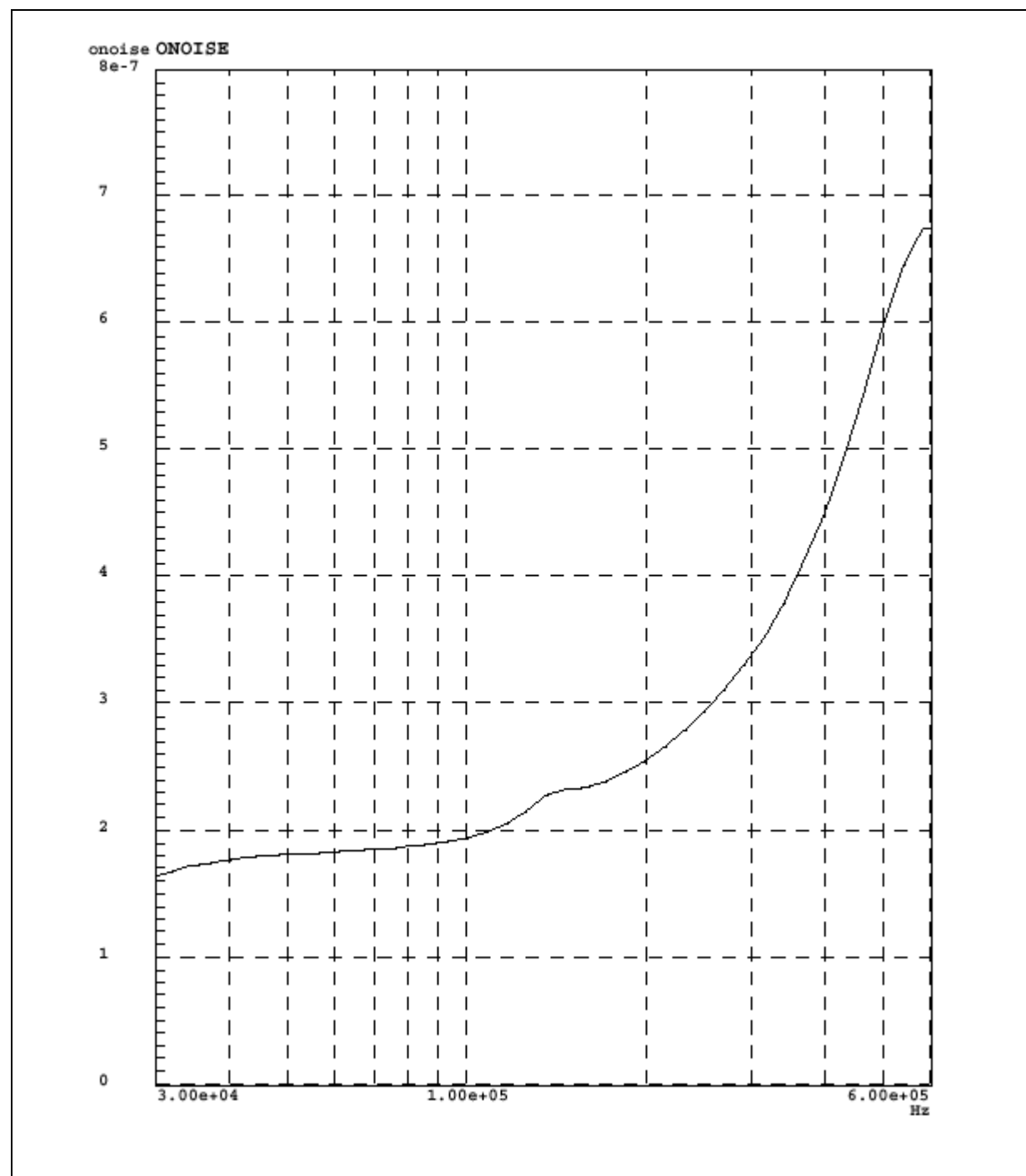
Figure 11. Total Transmit Path Noise Performance at the Line ( \text{nV}/\sqrt{\text{Hz}} )
