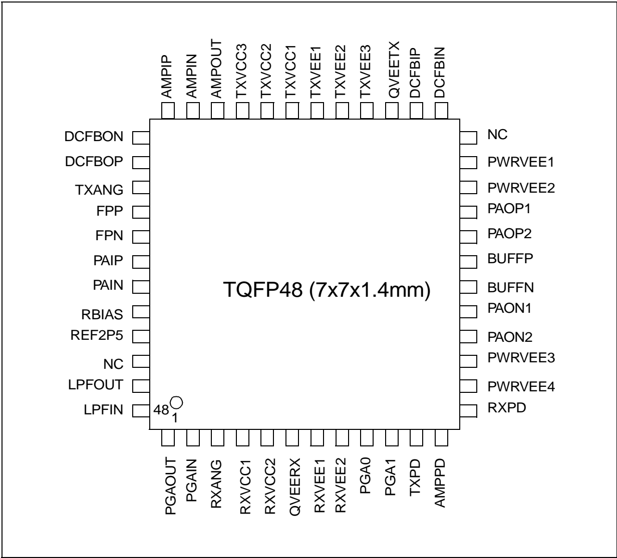
Figure 2. STLC1512 pinout
