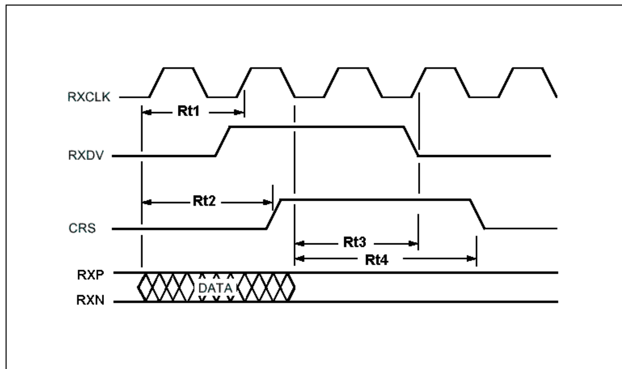
Figure 9. Receive Timing
