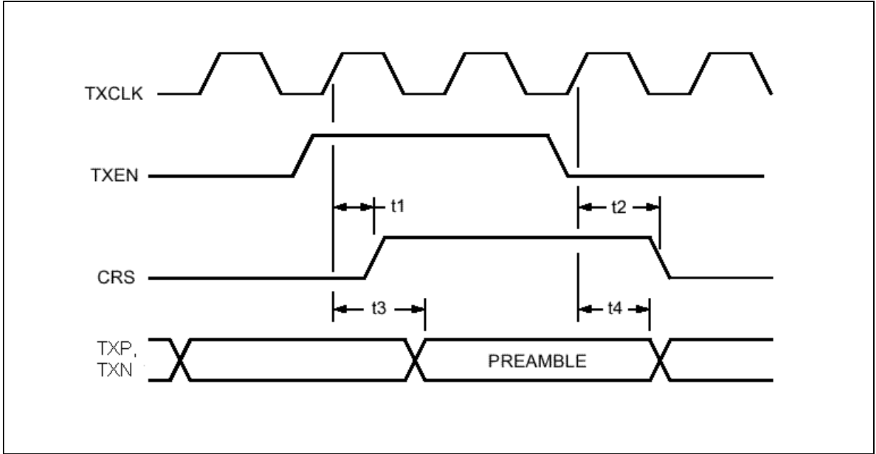
Figure 10. Transmit Timing
