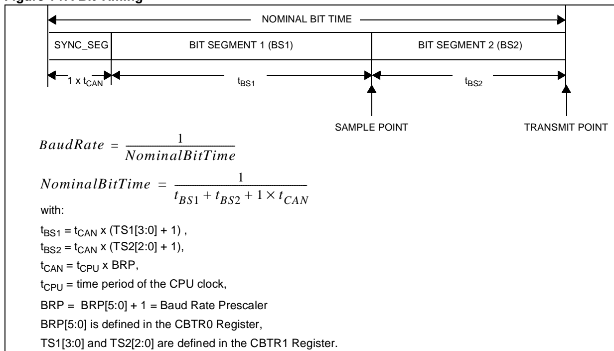
Figure 147. Bit Timing
