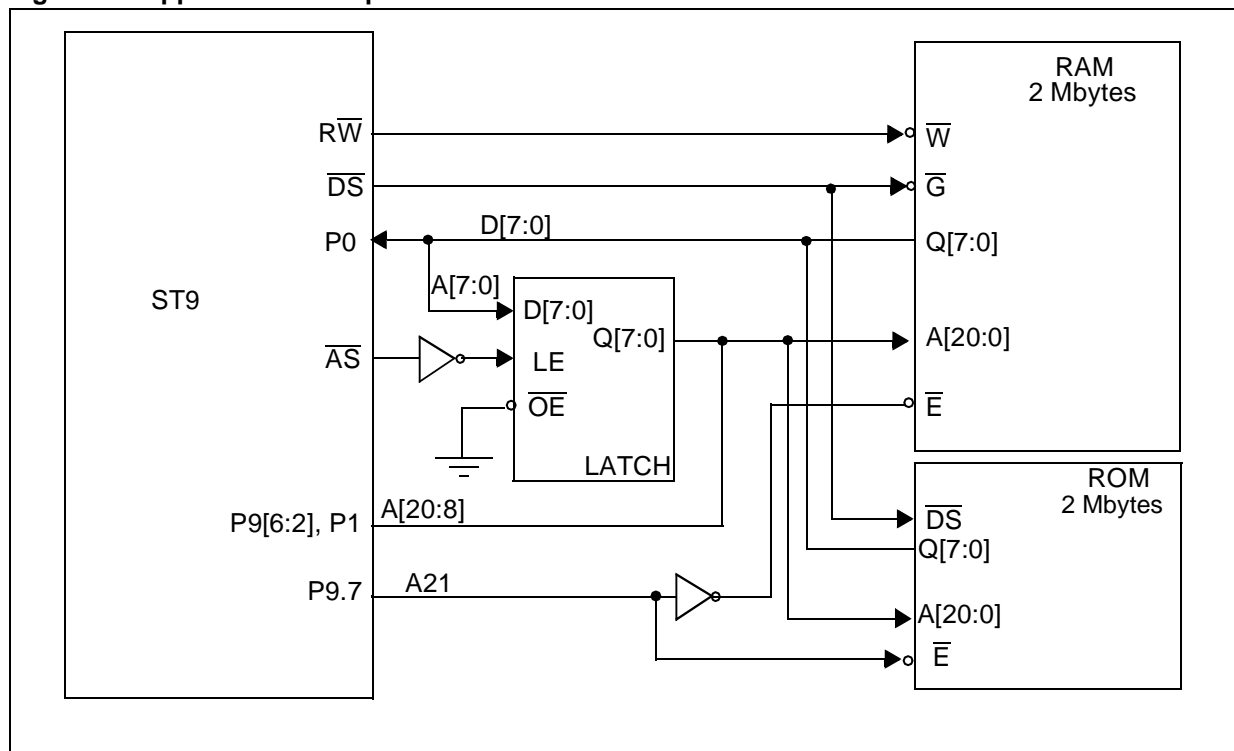
Figure 70. Application Example
