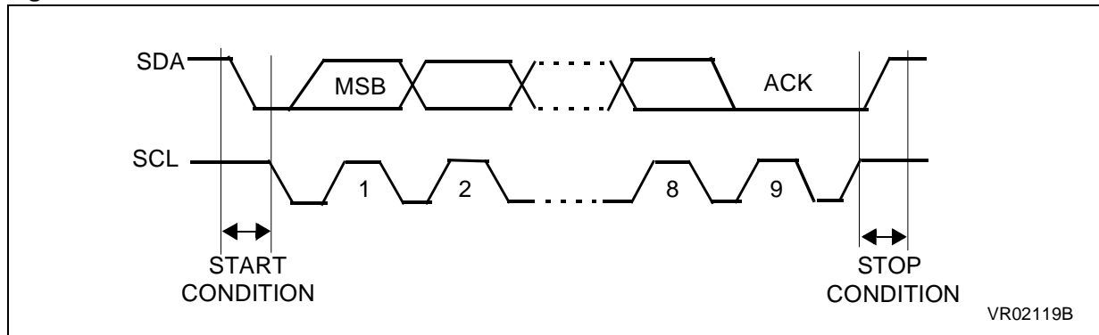
Figure 122. I 2 C BUS Protocol
