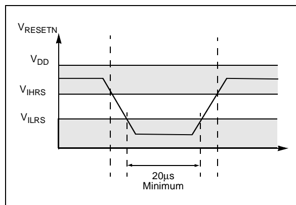
Figure 67. Recommended Signal to be Applied on Reset Pin
