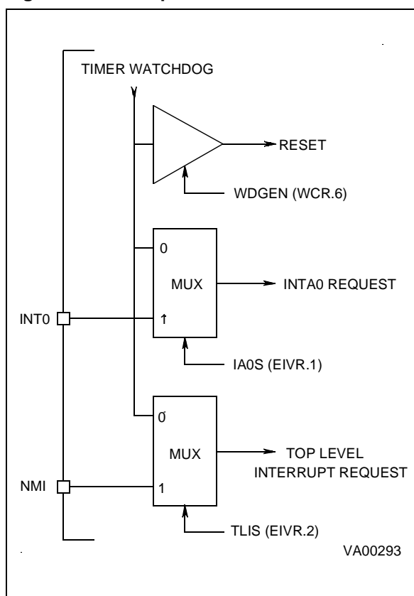
Figure 84. Interrupt Sources
