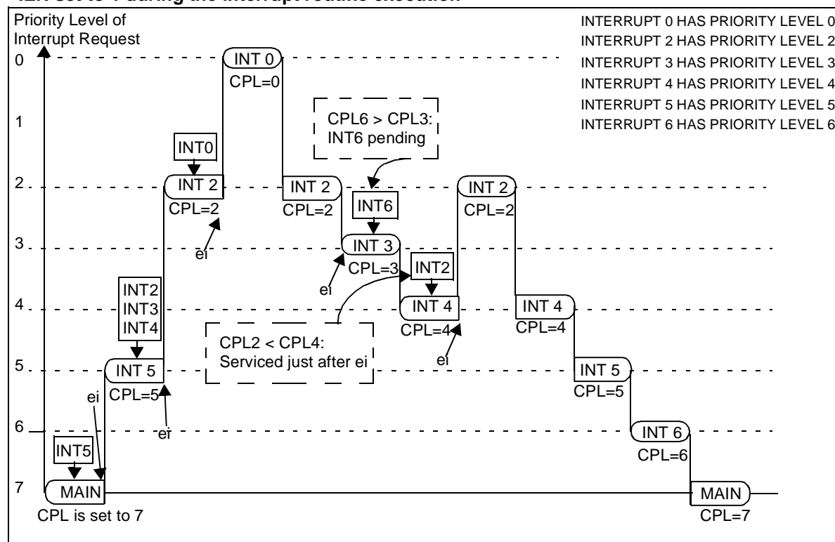
Figure 45. Complex Example of a Sequence of Interrupt Requests with:
