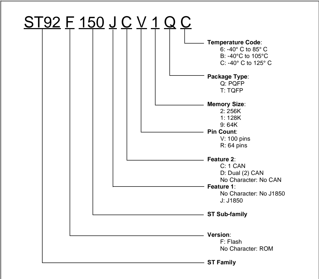
Figure 157. Device Types
