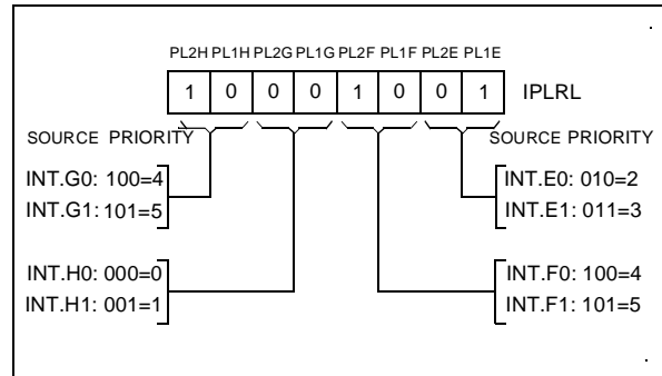
Figure 48. Priority Level Examples
