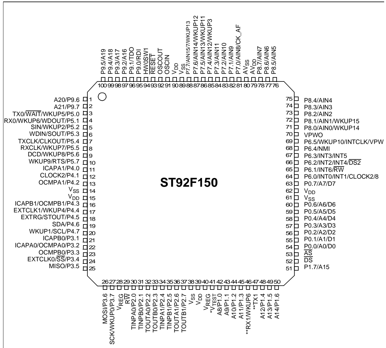
Figure 13. ST92F150: Pin Configuration (Top-view TQFP100)
