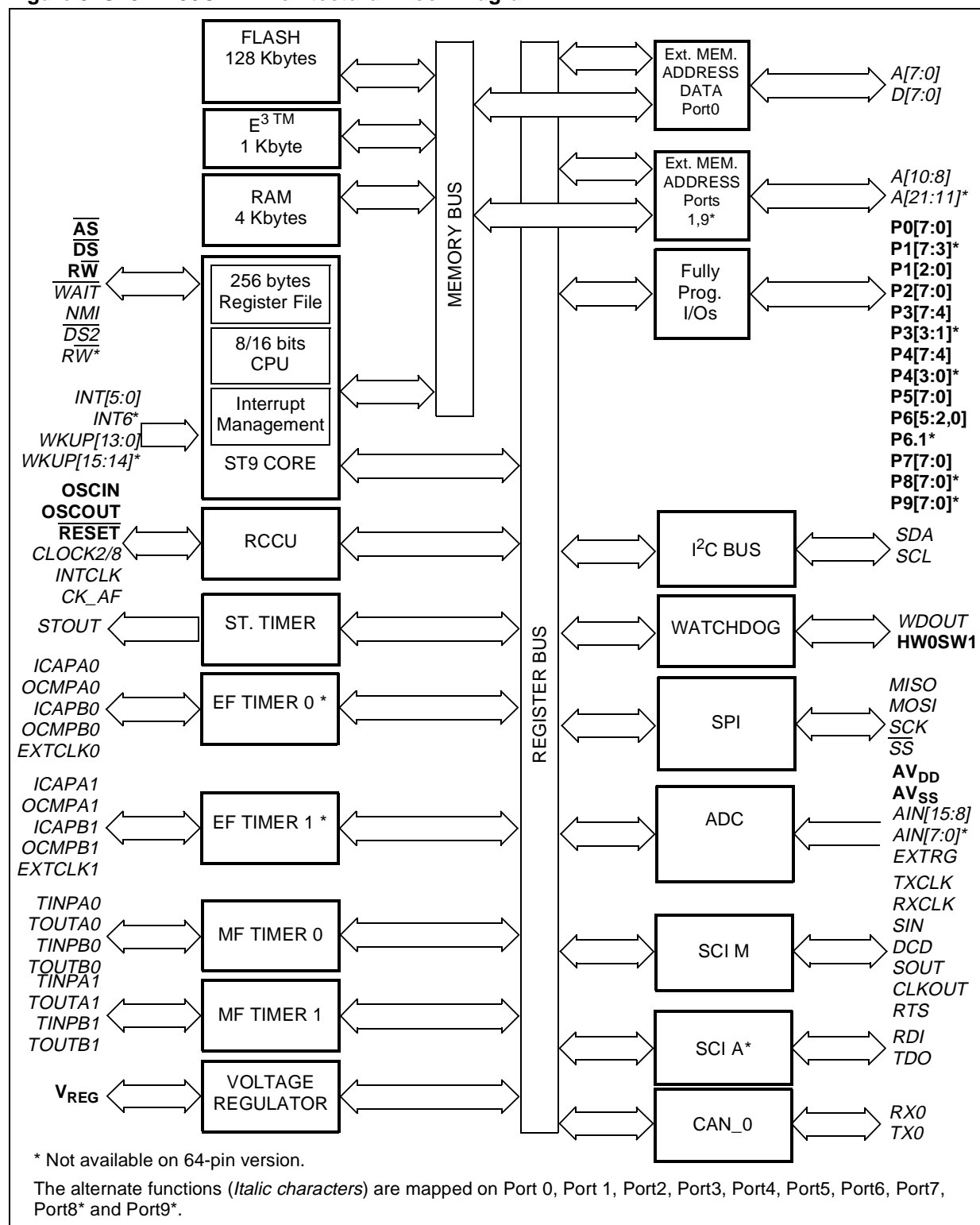
Figure 3. ST92F150CV1: Architectural Block Diagram
