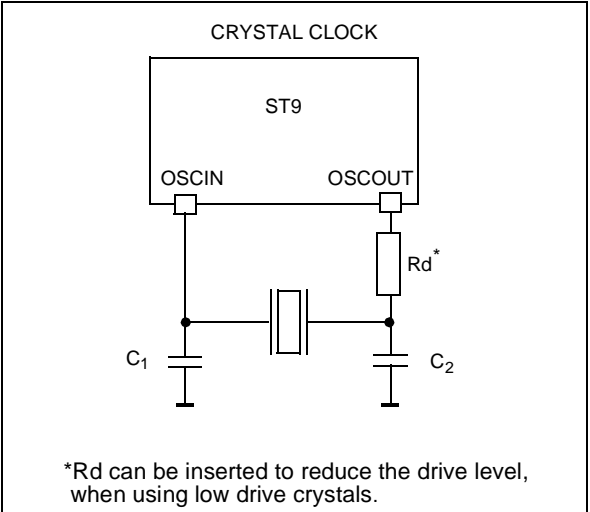
Figure 62. Crystal Oscillator
