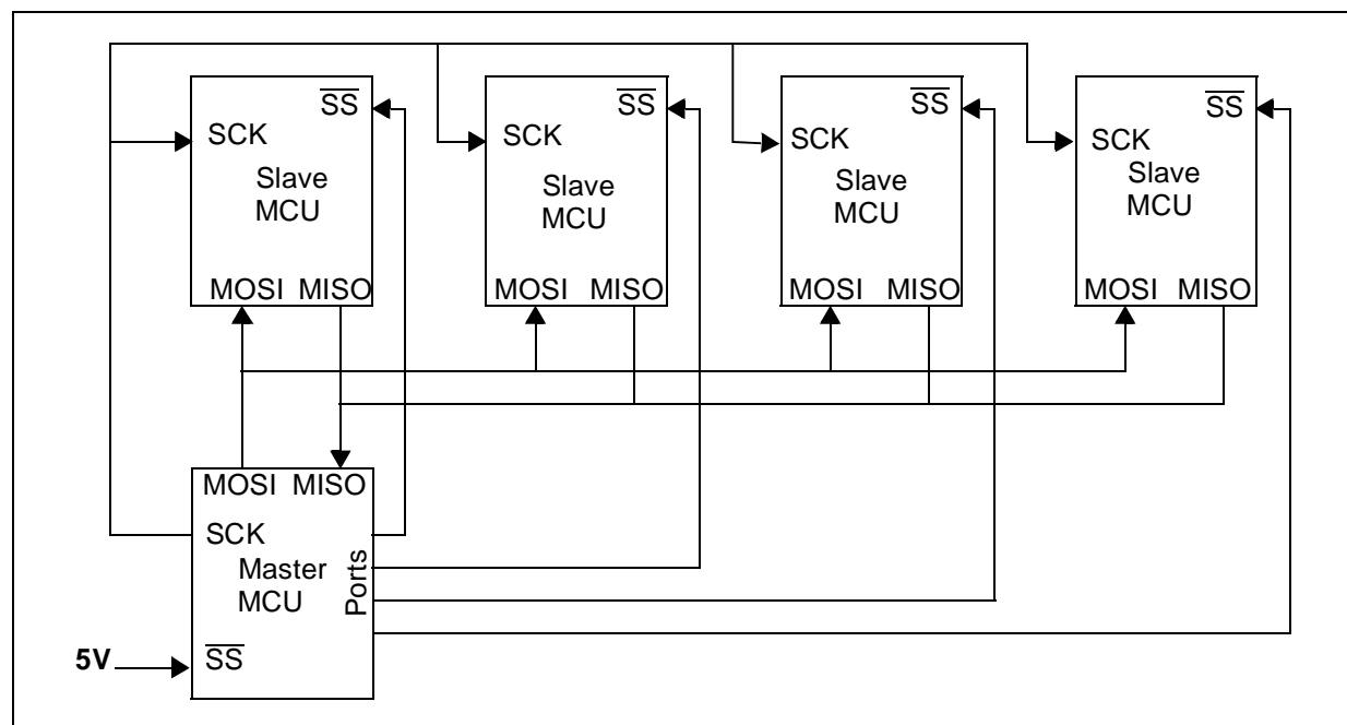
Figure 120. Single Master Configuration
