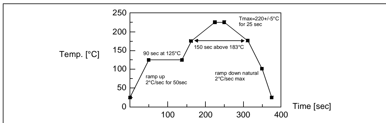
Figure 49. Recommended Reflow Oven Profile (MID JEDEC)
