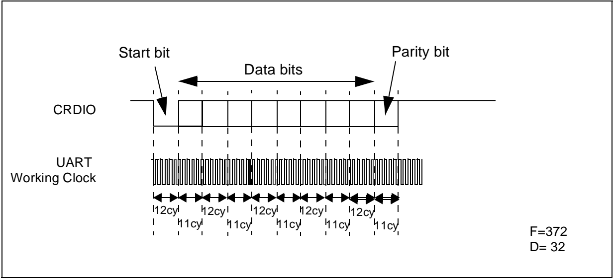
Figure 30. Compensation Mode
