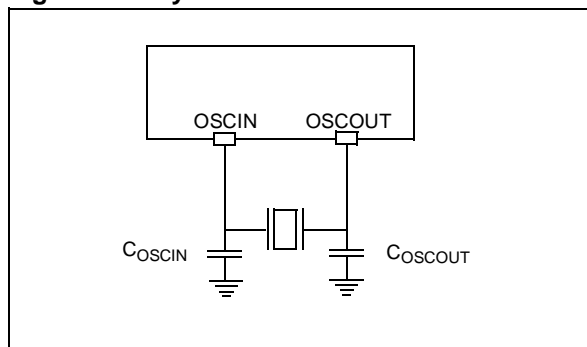
Figure 12. Crystal Resonator
