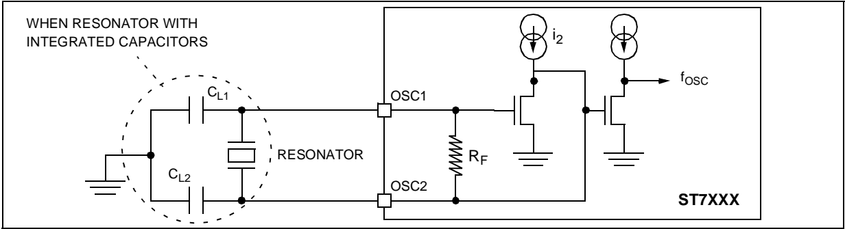
Figure 39. Typical Application with a Crystal Resonator
