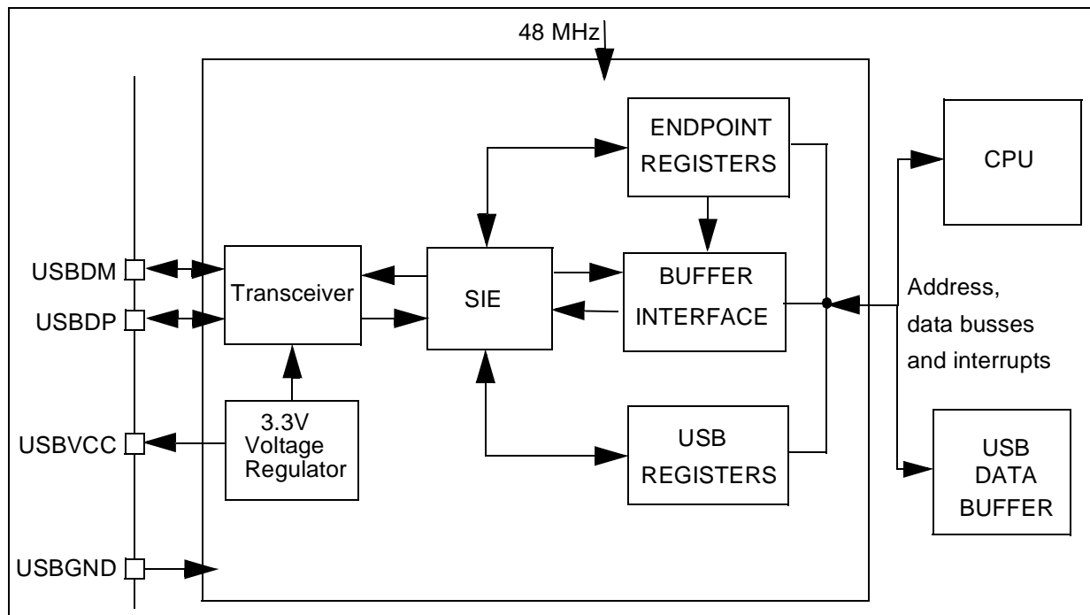
Figure 27. USB Block Diagram
