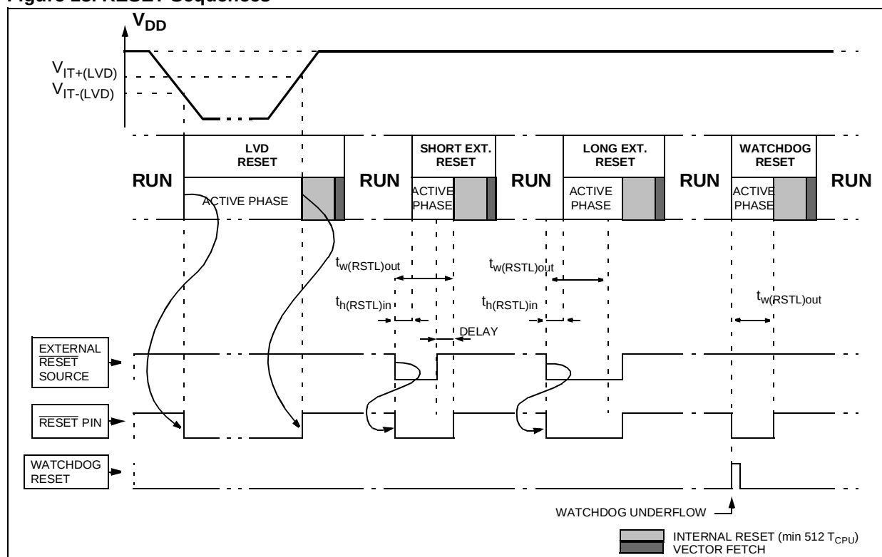
Figure 18. RESET Sequences
