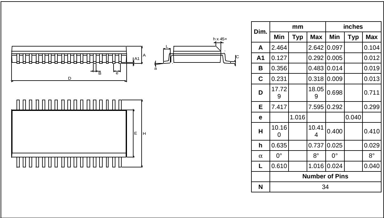
Figure 107. 34-Pin Plastic Small Outline Package, Shrink 300-mil Width
