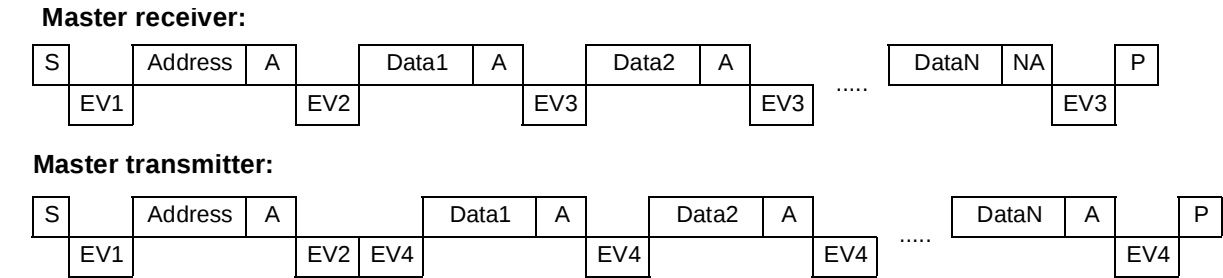
Figure 68. Transfer Sequencing
