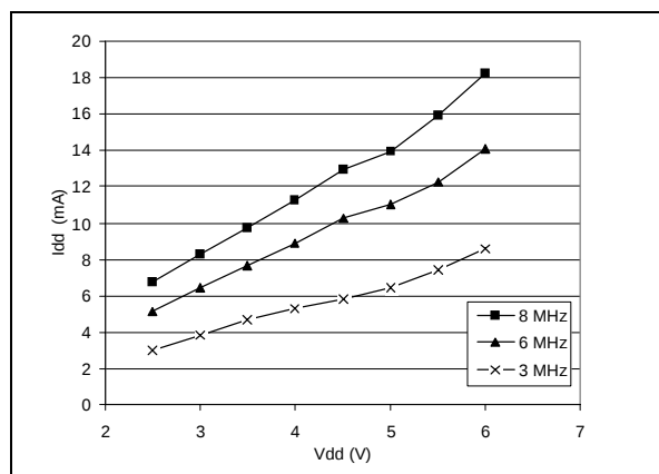
Figure 75. Typical I_{DD} in RUN vs. f_{CPU}
