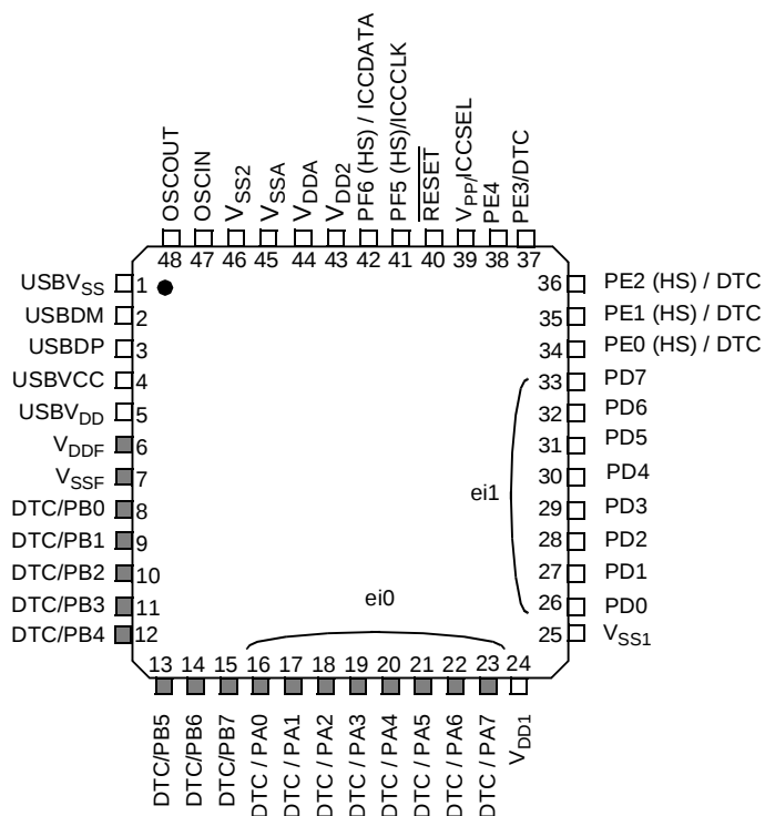
Figure 5. 48-Pin TQFP Package Pinout
