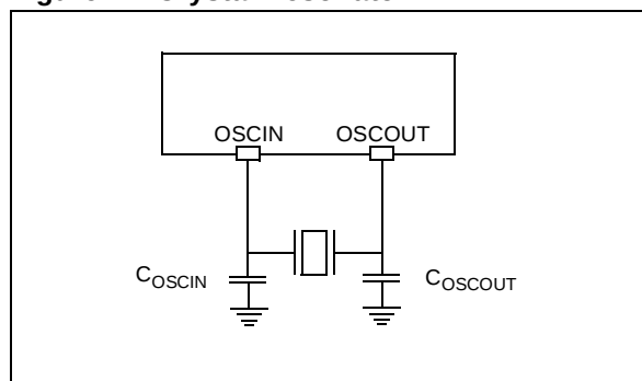
Figure 17. Crystal Resonator
