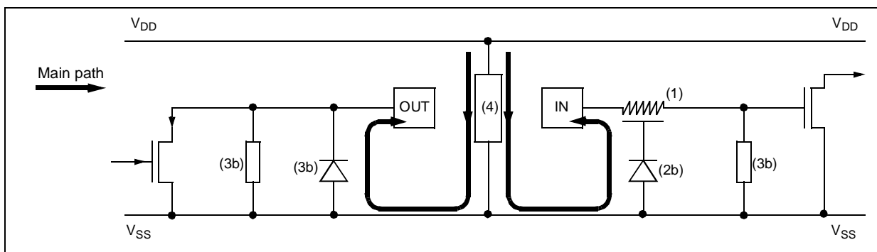
Figure 60. Multisupply Configuration
