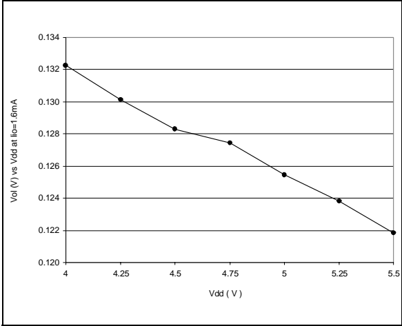
Figure 70. Typical V_{OL} vs. V_{DD} (very high-sink I/Os)
