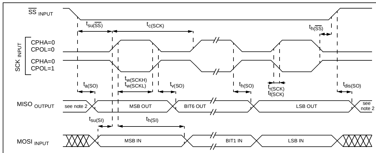
Figure 110. SPI Slave Timing Diagram with CPHA=0 3)
