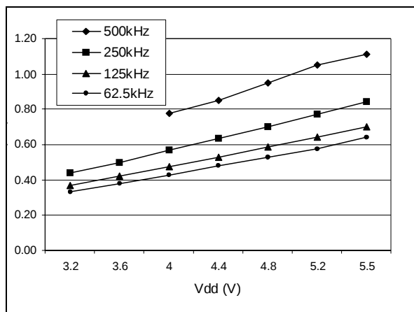
Figure 88. Typical I_{DD} in SLOW-WAIT vs. f_{CPU}
