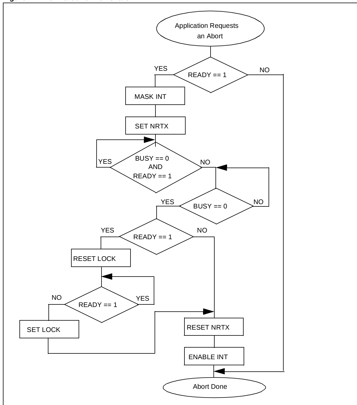
Figure 74. Work-around Flowchart
