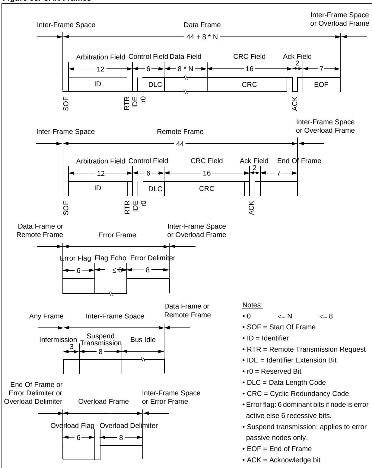
Figure 68. CAN Frames
