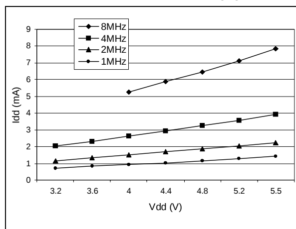
Figure 85. Typical I_{DD} in RUN vs. f_{CPU}
