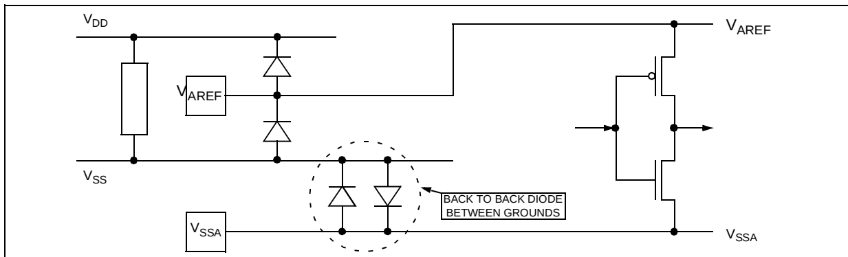
Figure 99. Multisupply Configuration
