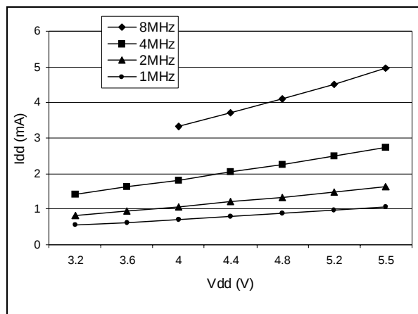
Figure 87. Typical I_{DD} in WAIT vs. f_{CPU}
