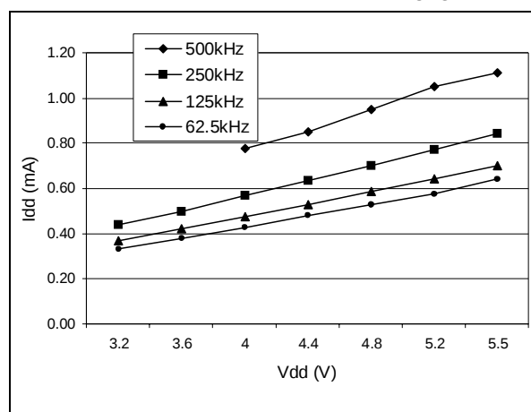
Figure 86. Typical I_{DD} in SLOW vs. f_{CPU}
