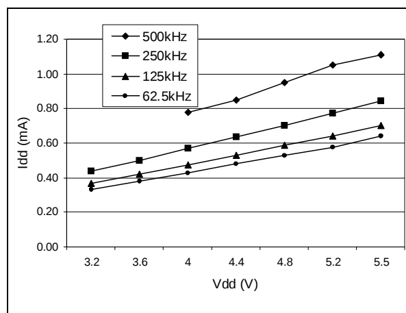
Figure 72. Typical I_{DD} in SLOW vs. f_{CPU}
