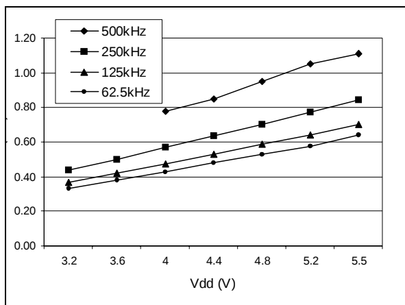
Figure 74. Typical I_{DD} in SLOW-WAIT vs. f_{CPU}
