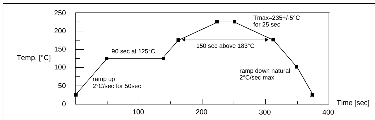
Figure 109. Recommended Reflow Soldering Oven Profile (MID JEDEC)
