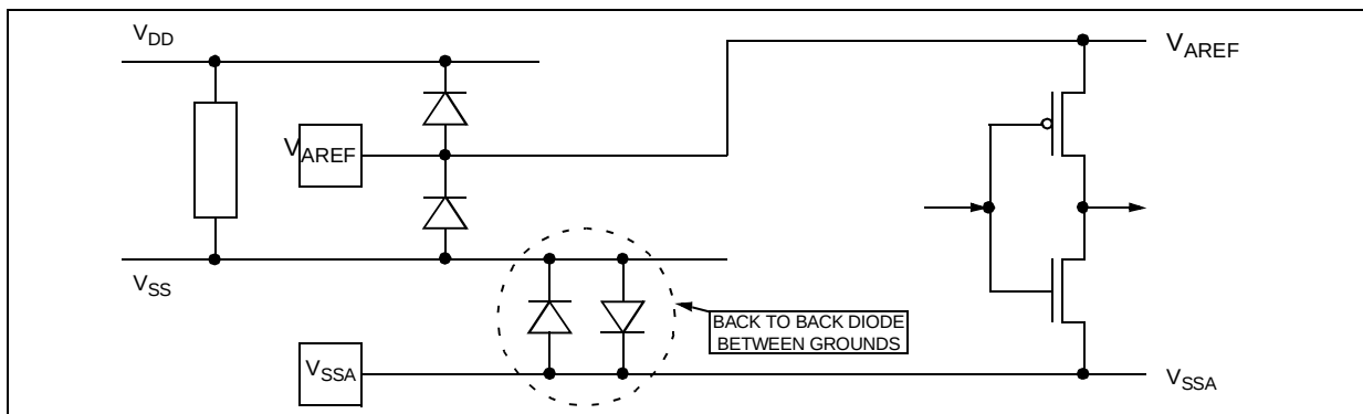
Figure 85. Multisupply Configuration
