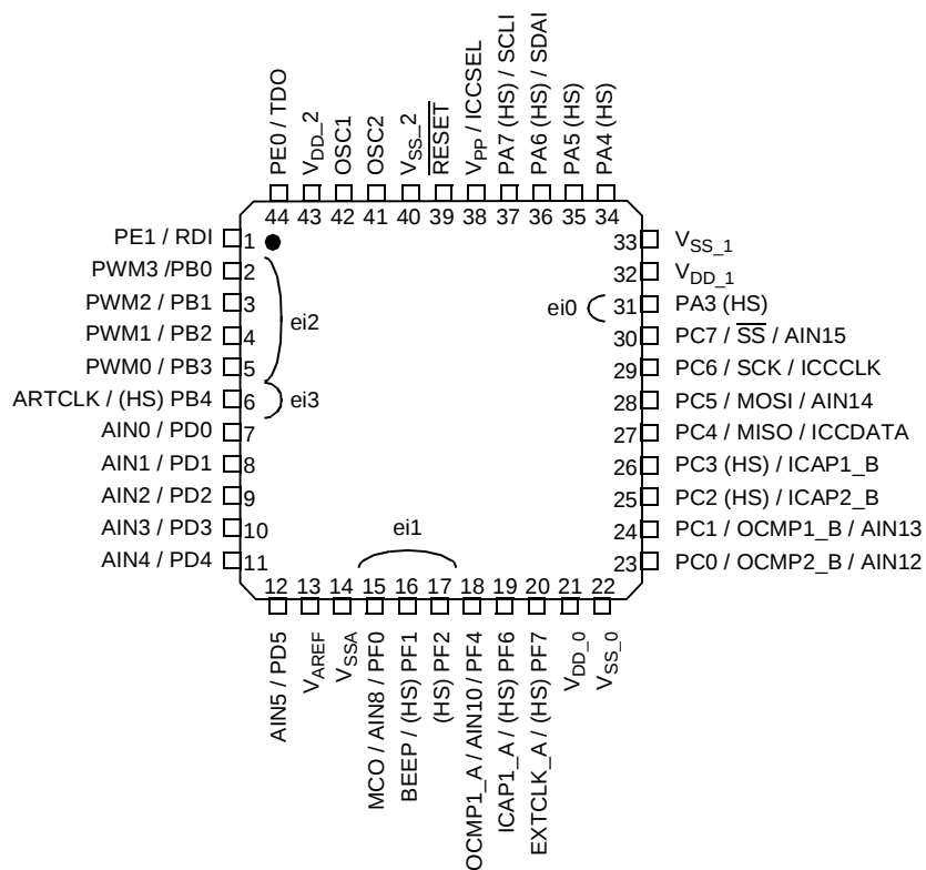
Figure 3. 44-Pin Device Pinout
