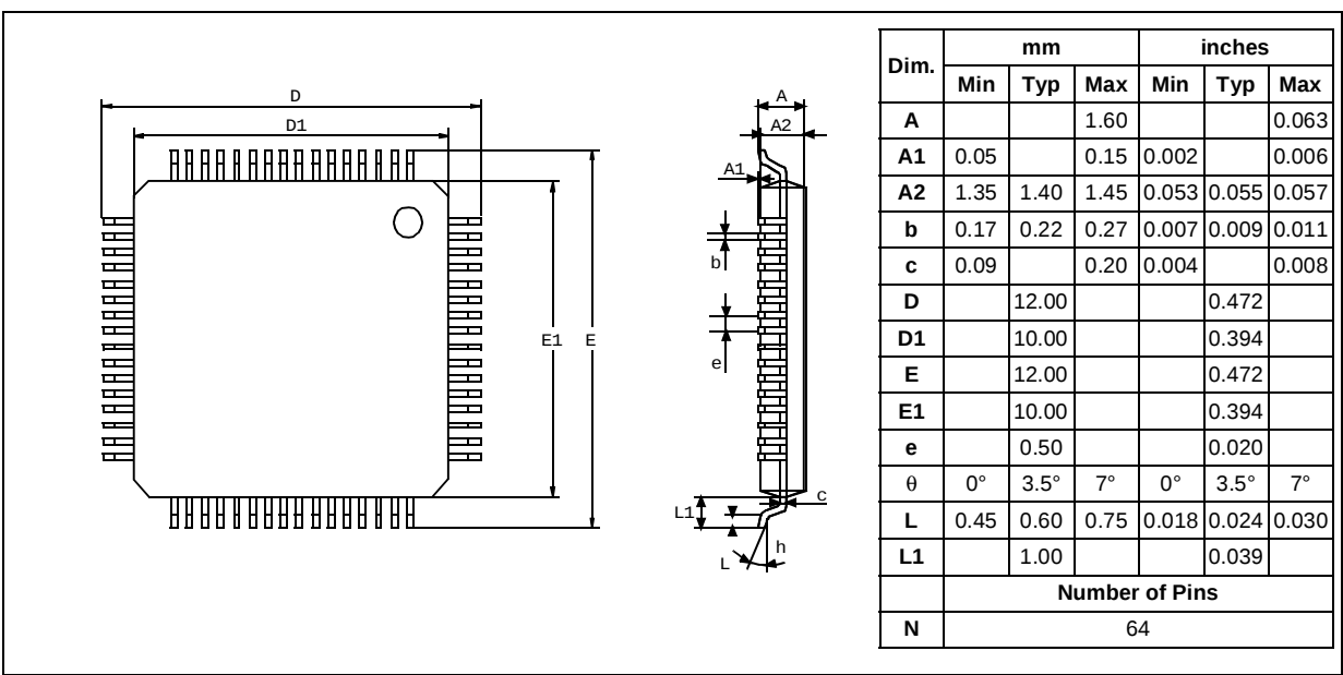
Figure 106. 64-Pin Thin Quad Flat Package
