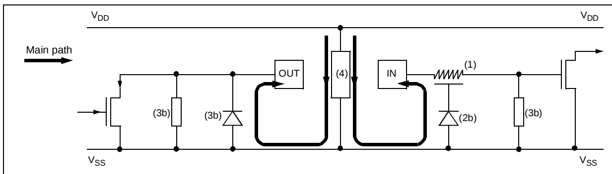
Figure 85. Multisupply Configuration
