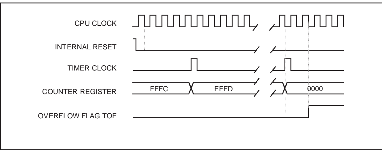
Figure 23. Counter Timing Diagram, internal clock divided by 8
