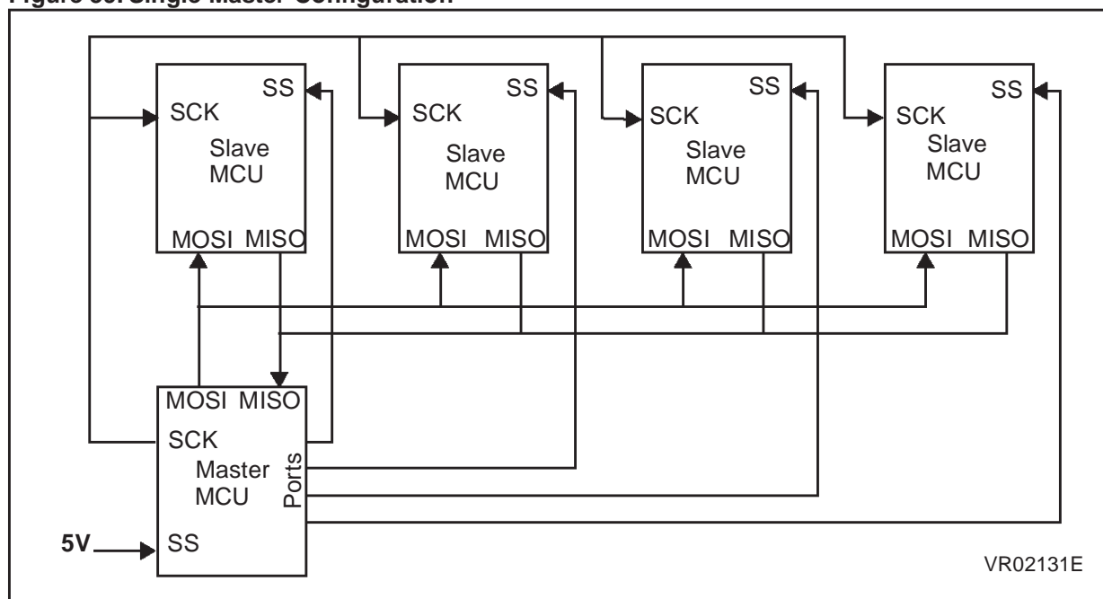
Figure 39. Single Master Configuration
