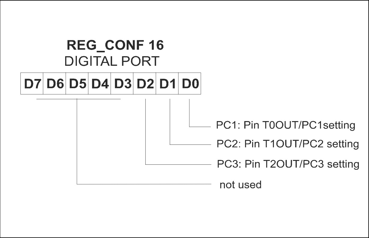
Figure 10.13 Configuration Register 16
