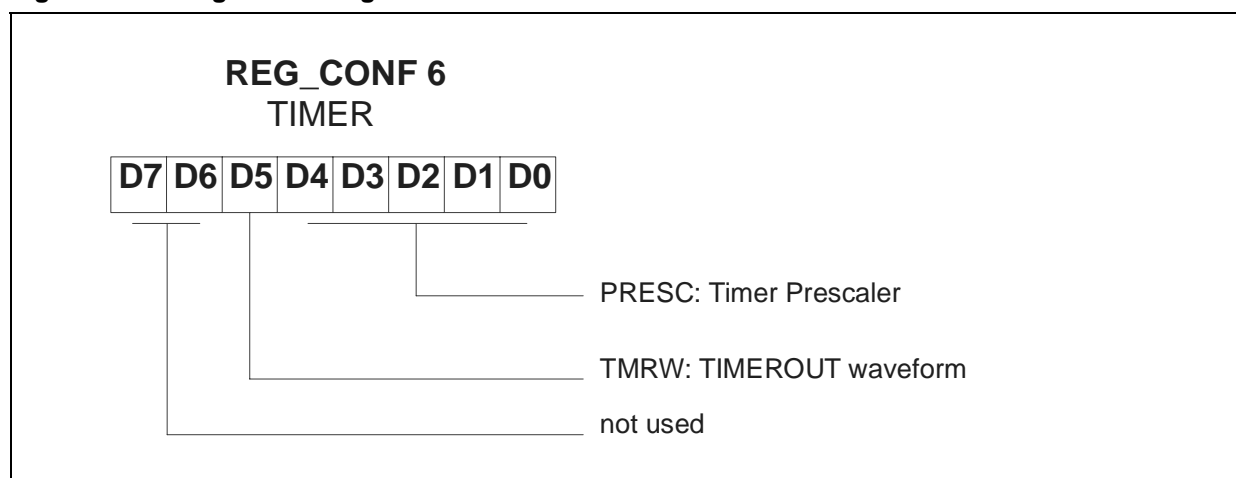
Figure 9.6 Configuration Register 6
