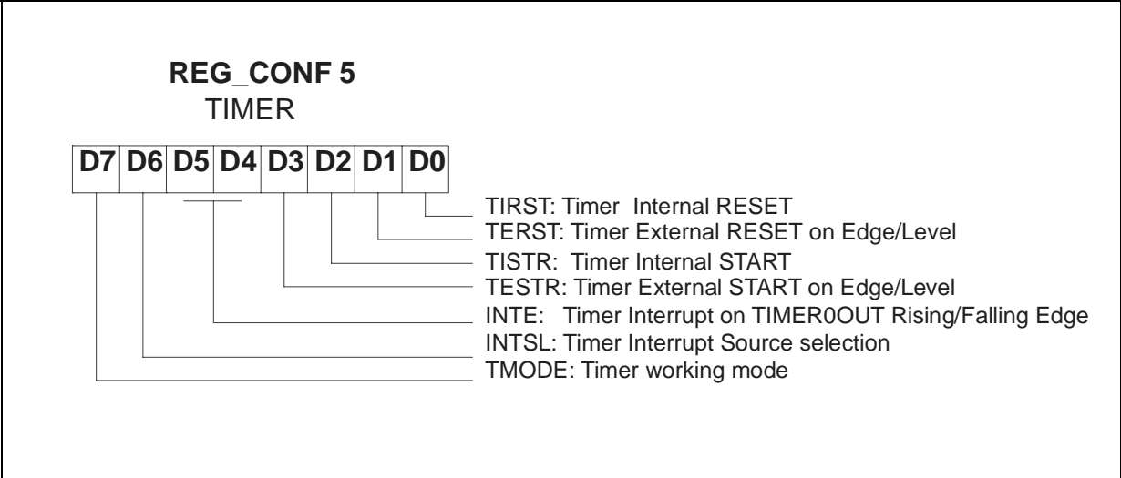
Figure 9.5 Configuration Register 5
