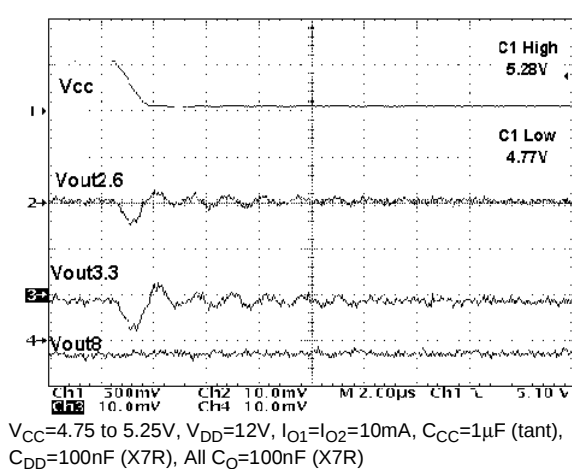
Figure 30 : Line Transient
