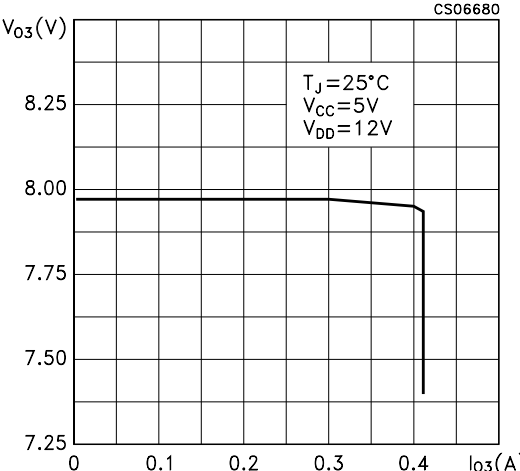
Figure 18 : Output Voltage vs Output Current
