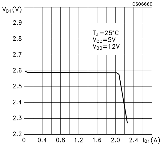
Figure 17 : Output Voltage vs Output Current
