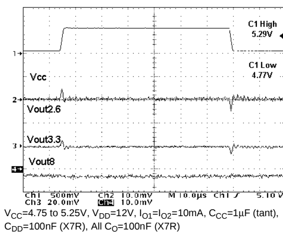
Figure 29 : Line Transient
