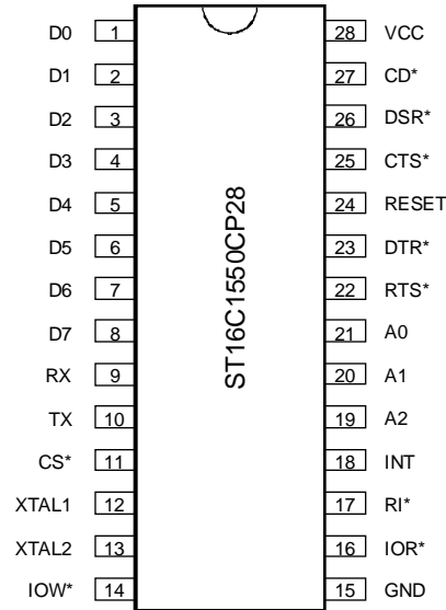
28 PIN PLASTIC-DIP ST16C1550
