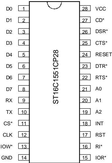
28 PIN PLASTIC-DIP ST16C1551
