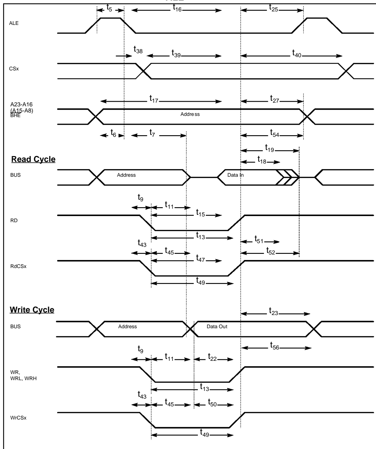
Figure 14.7 External Memory Cycle: Multiplexed Bus, No Read/Write Delay, Normal ALE
