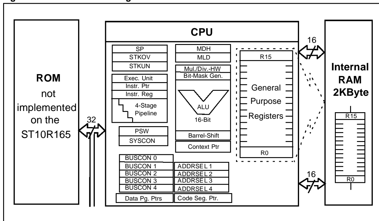
Figure 6.1 CPU Block Diagram
