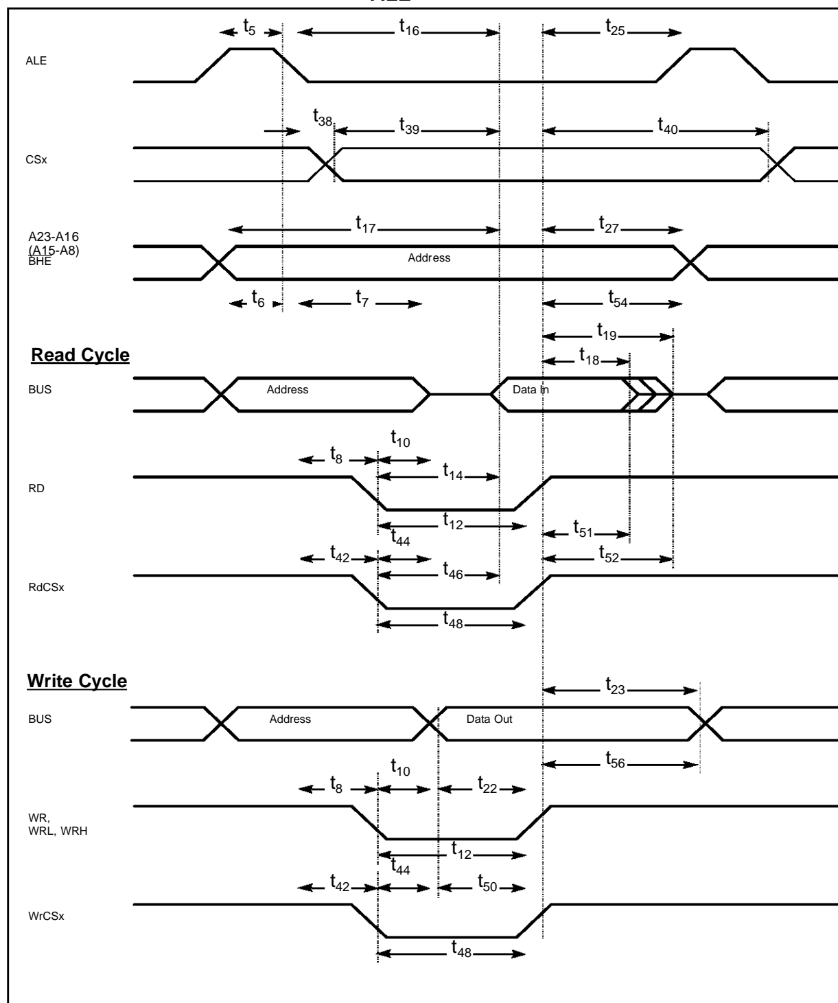
Figure 14.5 External Memory Cycle: Multiplexed Bus, With Read/Write Delay, Normal ALE
