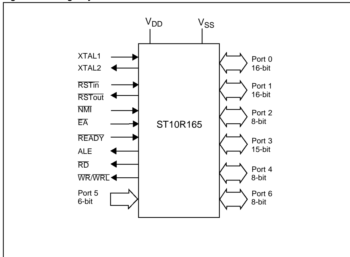
Figure 1.1 Logic Symbol
