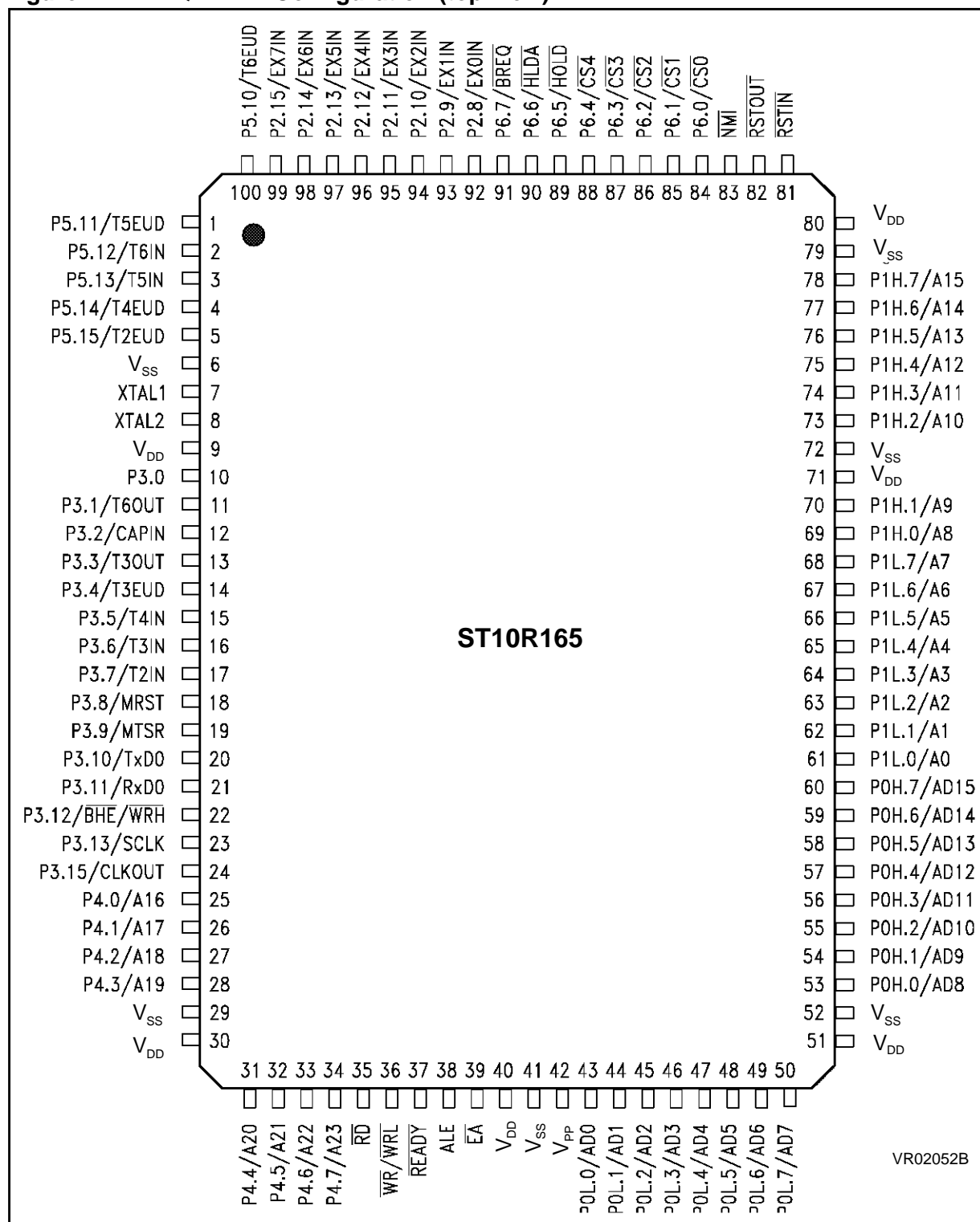
Figure 2.1 PQFP Pin Configuration (top view)
