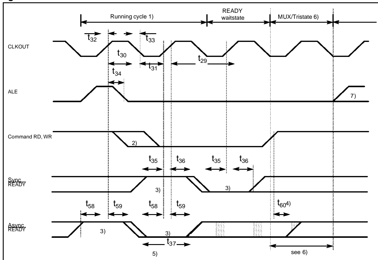
Figure 14.13 CLKOUT and \overline{\text{READY}}
