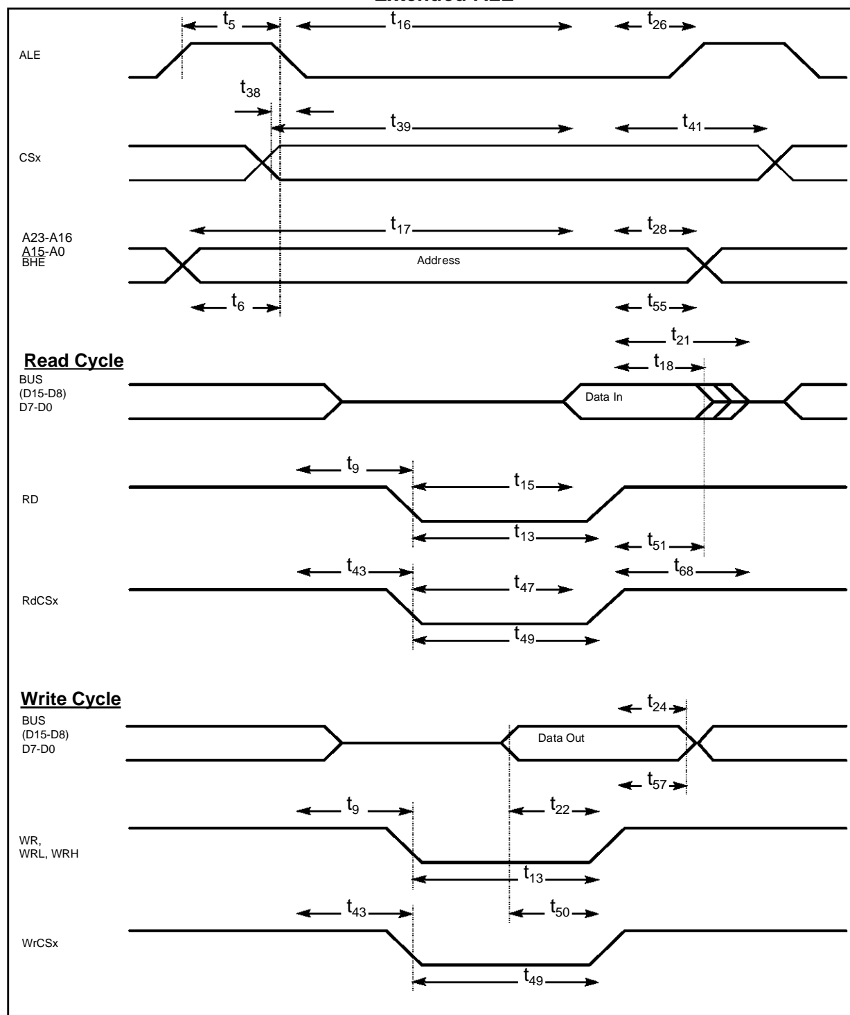
Figure 14.12 External Memory Cycle: Demultiplexed Bus, No Read/Write Delay, Extended ALE
