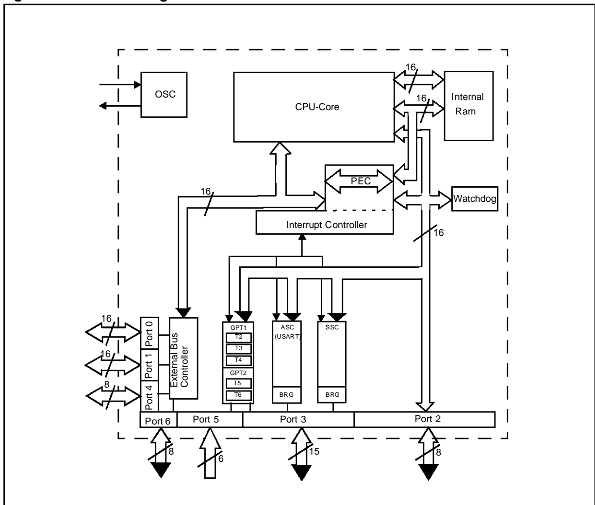
Figure 3.1 Block Diagram
