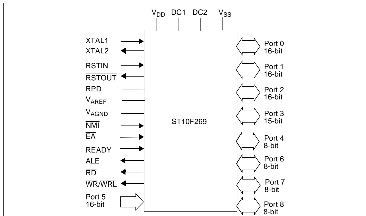
Figure 1 : Logic Symbol
