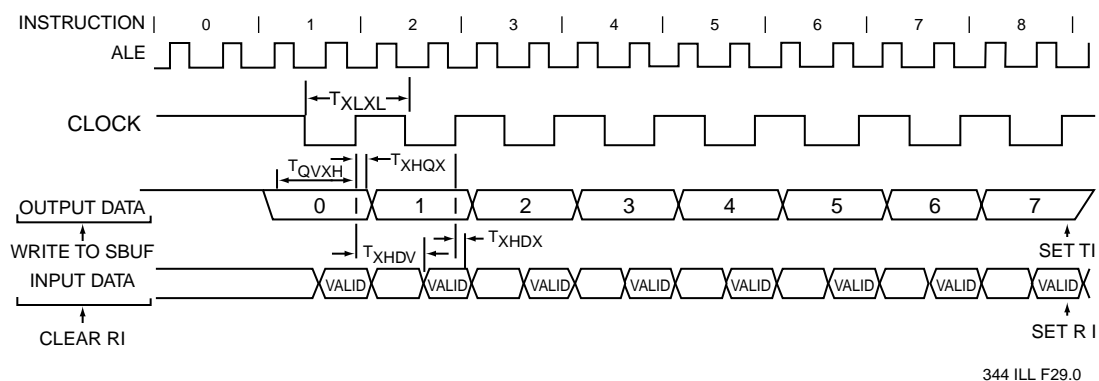
FIGURE 31: SHIFT REGISTER MODE TIMING WAVEFORMS
