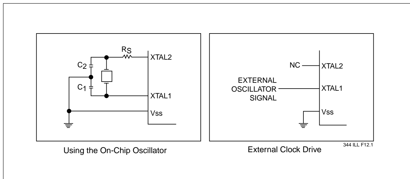
FIGURE 21: OSCILLATOR CHARACTERISTICS
