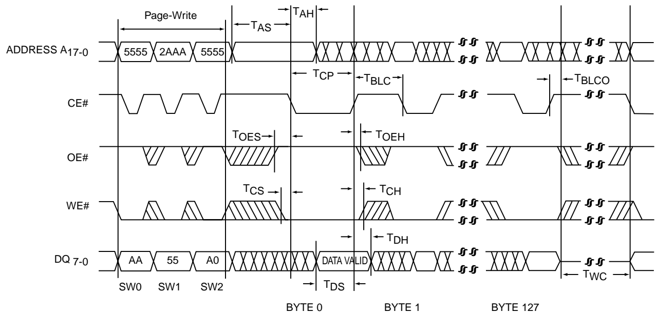
FIGURE 5: CE# CONTROLLED PAGE-WRITE CYCLE TIMING DIAGRAM
