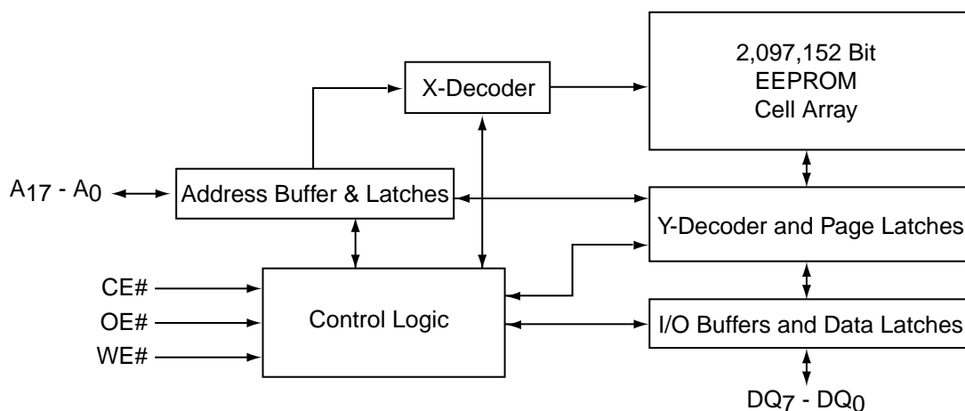
FUNCTIONAL BLOCK DIAGRAM OF SST 29EE020A/29LE020A/29VE020A
