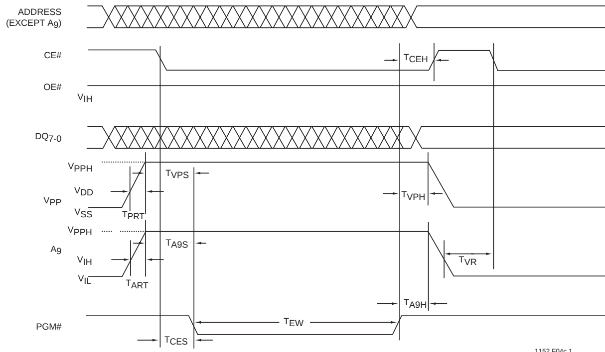
FIGURE 6: CHIP-ERASE TIMING DIAGRAM FOR SST27SF010/020
