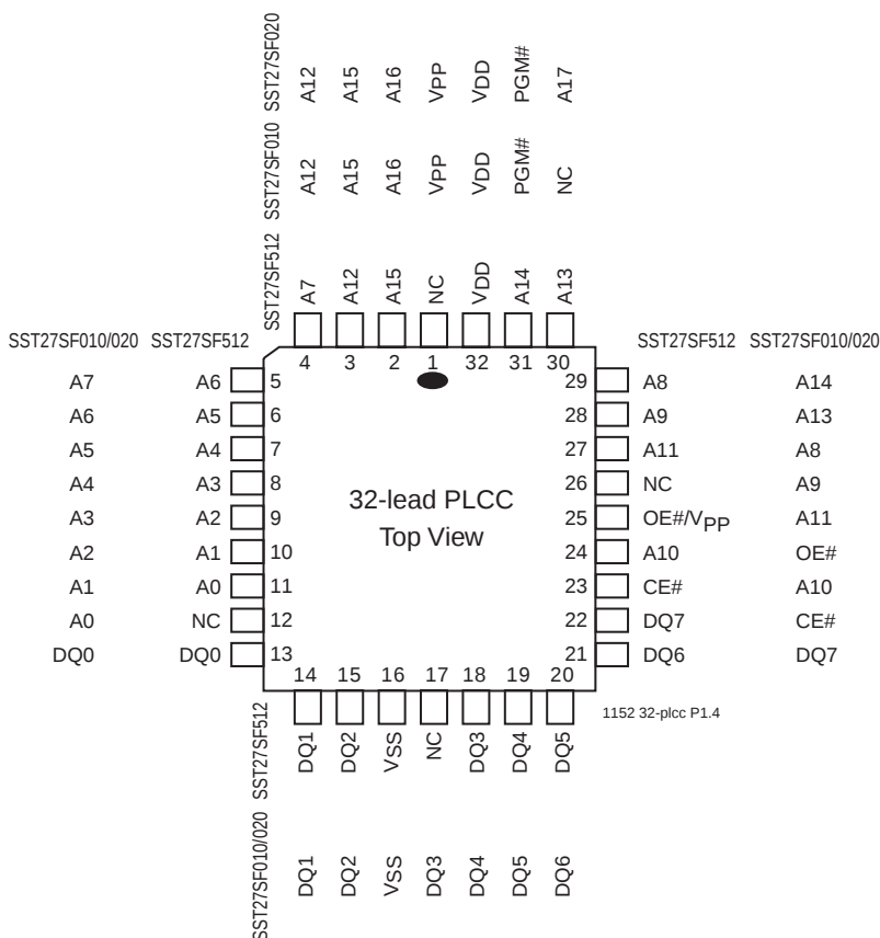
FIGURE 1: PIN ASSIGNMENTS FOR 32-LEAD PLCC
