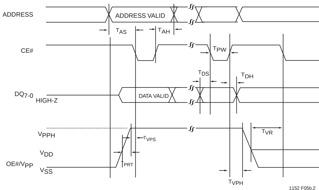
FIGURE 7: BYTE-PHASE TIMING DIAGRAM FOR SST27SF512
