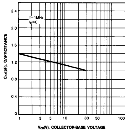
OUTPUT CAPACITANCE
