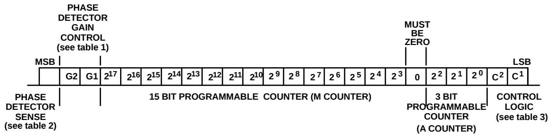
Fig. 7(b) F1 or F2 word, bit allocation with 8/9 selected
