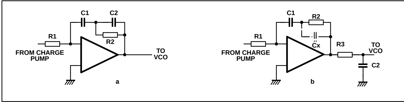
Fig. 11 Third order loop filter
