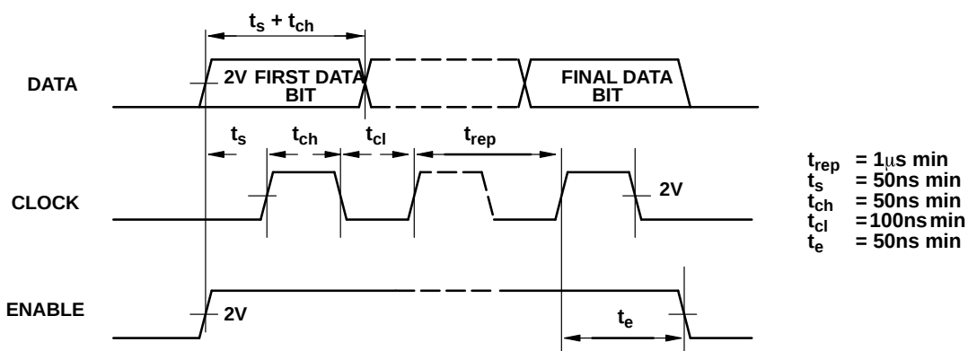
Fig. 5 Data and clock timing requirements
