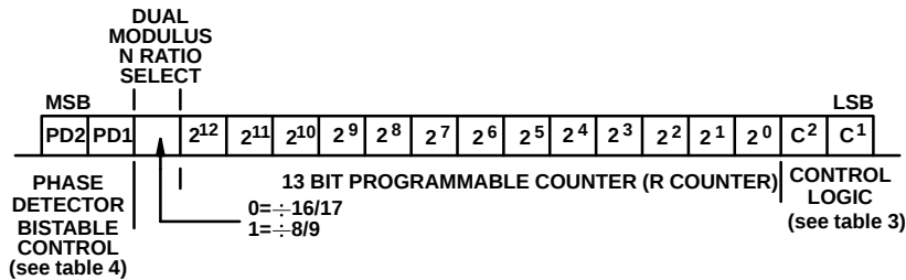
Fig. 7(c) Reference word bit allocation
