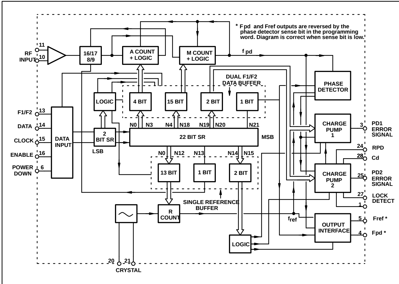
Fig. 2 SP8861 block diagram
