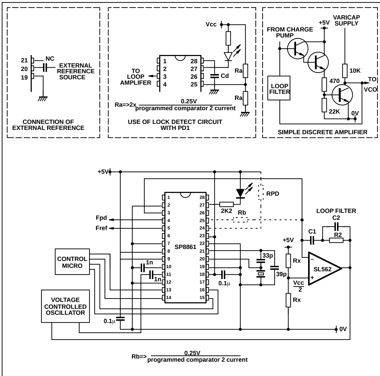
Fig. 6 Typical application diagram
