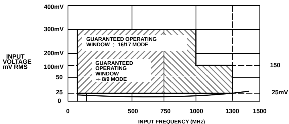
Fig.4 Typical input characteristics and input drive requirements
