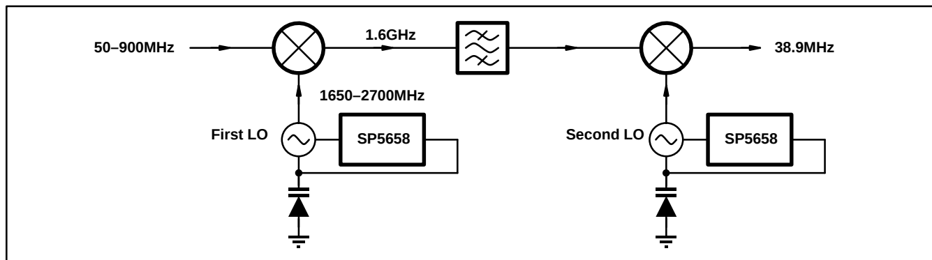
Fig. 6 Example of double conversion from VHF/UHF frequencies to TV IF
