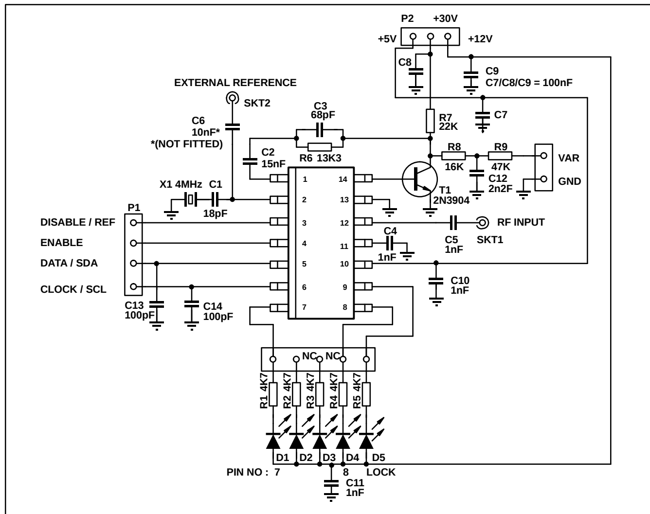
Fig. 8 Test board
