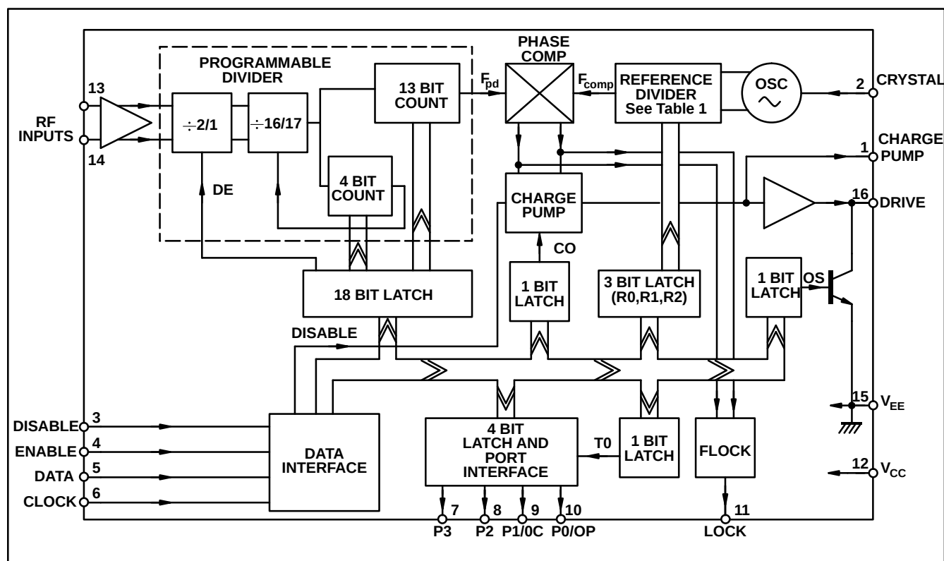
Fig. 2 SP5658S block diagram
