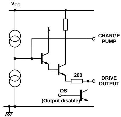
Loop amplifier
