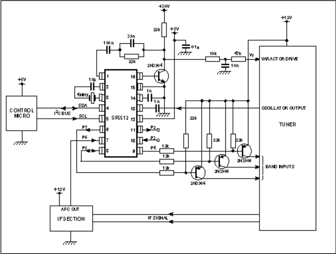
Fig. 4 Typical application
