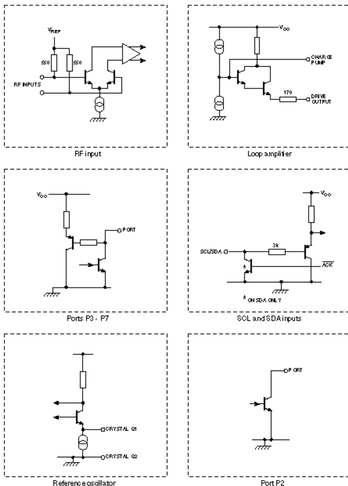
Fig. 6 Input/output interface circuits
