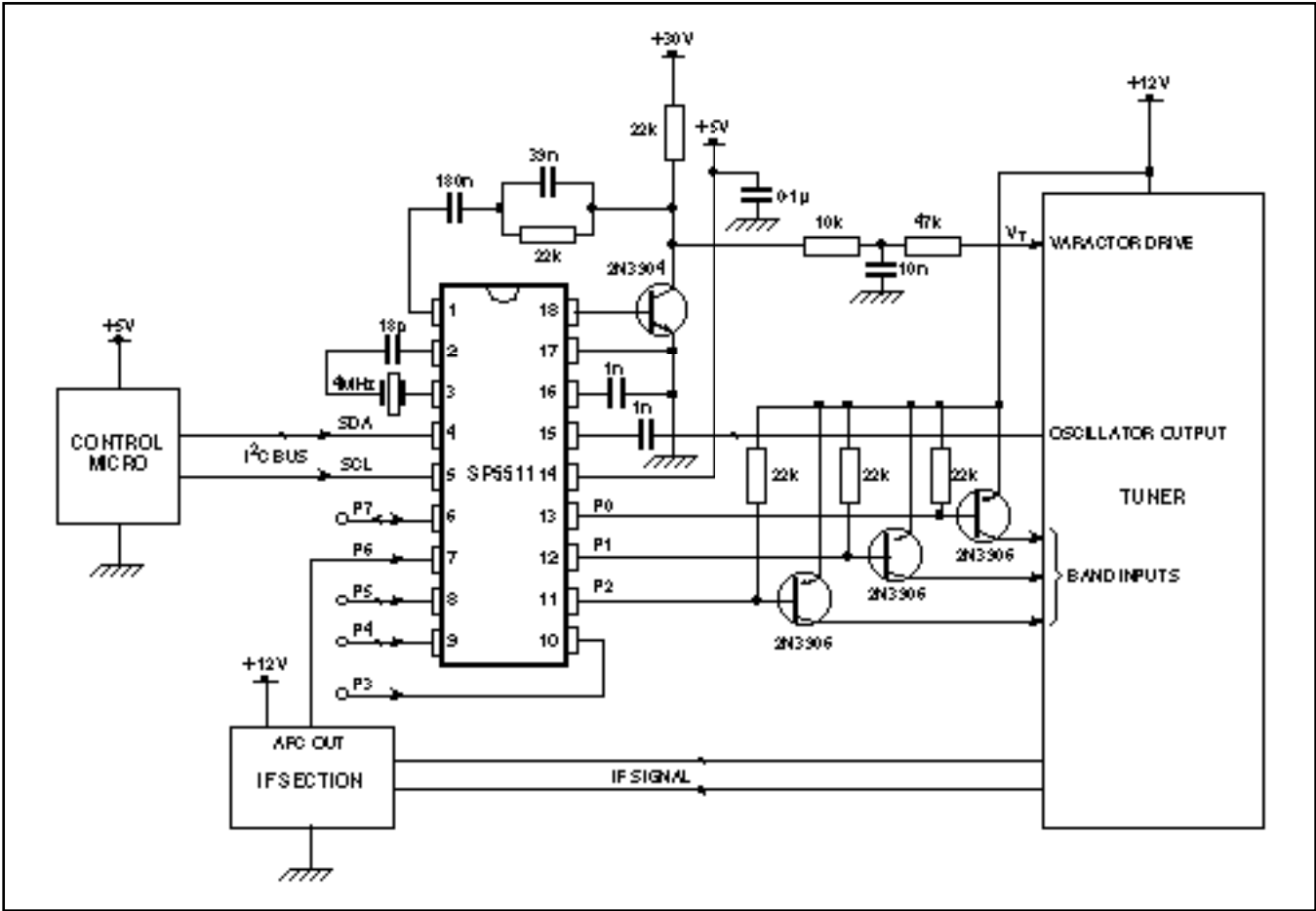
Fig. 4 Typical application
