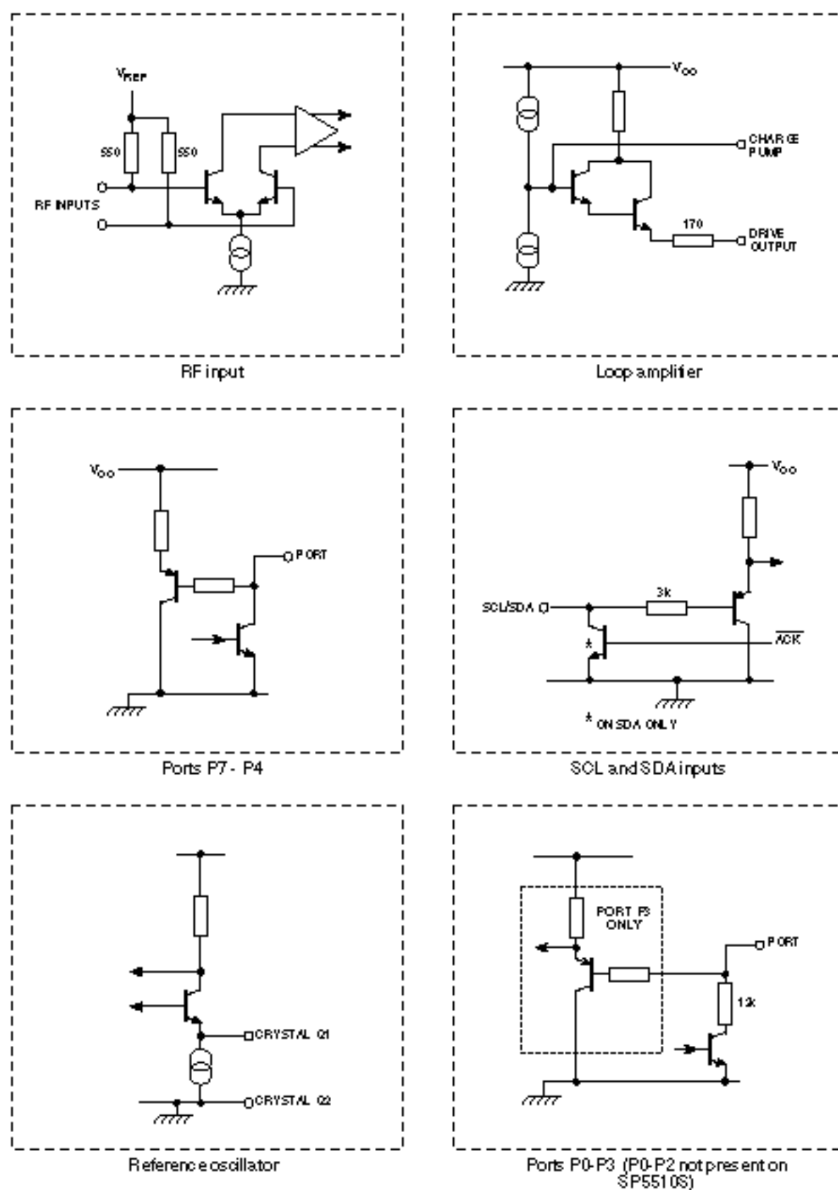
Fig. 6 SP5510 input/output interface circuits
