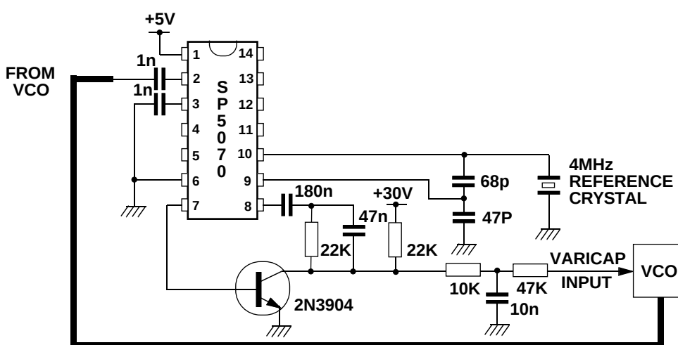
Fig.3 Typical application and test circuit (1024MHz with 4MHz reference crystal)
