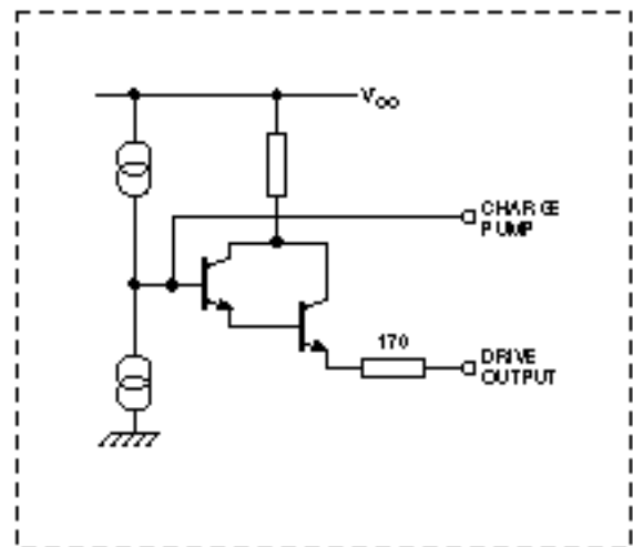
Loop amplifier
