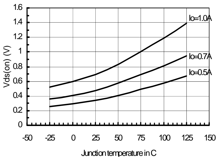
Normalized FET on resistance
