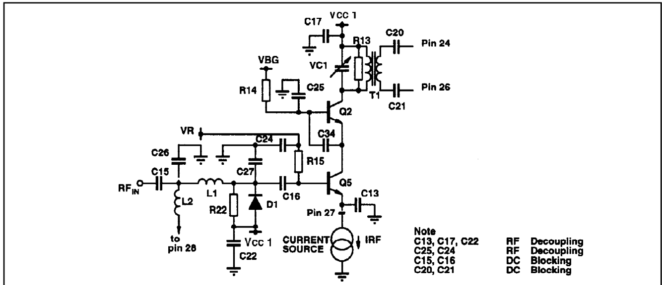
Fig.4 RF amplifier
